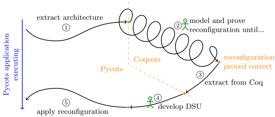
Figure 3: Overview of the proposed approach.
