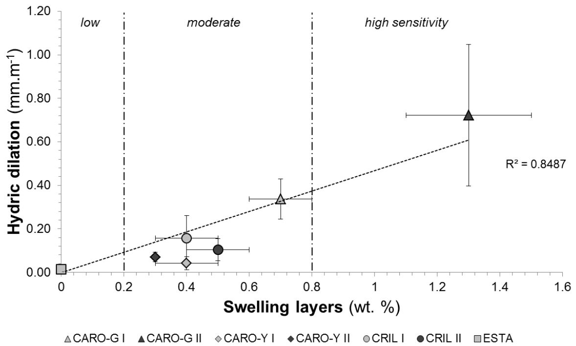
Figure 6. Mean hydic dilatation coefficients of the seven studied samples as a function of their amounts of swelling layers. The limits between low, moderate, and high sensitivity to spalling decay were placed according to [13].
