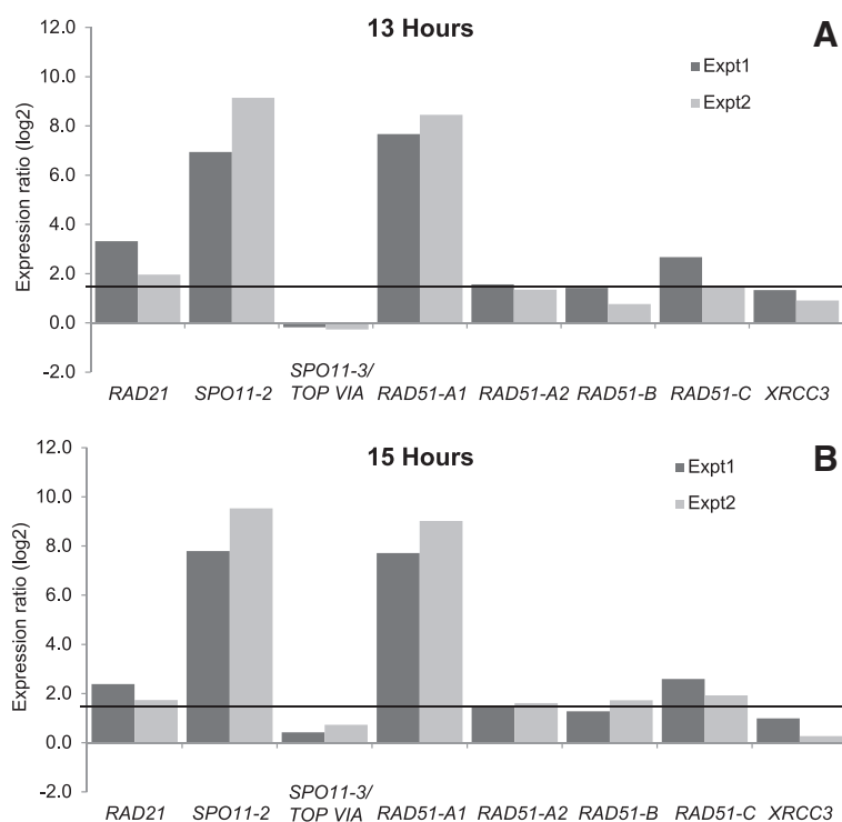
Fig. 5 Differential expression analysis of RAD21 , SPO11 and RAD51 homologs during meiosis in Pseudo-nitzschia multistriata . Two time points, 13 h (a) and 15 h (b) after strains of opposite mating type were mixed together, were selected for expression analyses. Dark gray bars represent experiment 1 (Expt1, B937 (MT+) with B936 (MT-)) and light gray bars represent experiment 2 (Expt2, B938 (MT+) with B939 (MT-)). Relative fold changes, with respect to vegetatively growing cultures, in log 2 scale, are reported on the Y-axis. A gene was considered differentially expressed if its relative expression change is 1.5 fold or greater (horizontal black line)
