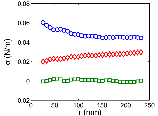
Fig. 11. Elastic stress components \sigma_{rr} (circles), \sigma_{\theta\theta} (lozenges) and \sigma_{r\theta} (squares) as a function of r , along the central axis \theta = 0 .
