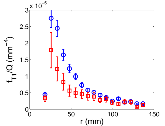
Fig. 15. Plot of the ratio of the T1 frequency to the foam flow rate as a function of r , for the experiment with the SDS solution (circles) and the SLES/CAPB/LAc mixture (squares).
