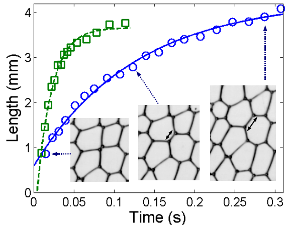
Fig. 13. Evolution of the length of a film created after a T1, for the SDS solution (squares) and the SLES/CAPB/LAc mixture (circles), and three snapshots of this film, represented by a double arrow. The time origin was chosen as the first image where this length could be measured reliably. The data were fitted by an exponential relaxation of the form \ell(t) = \ell_1 + \ell_2 e^{-(t-t_0)/\tau_r} , with \ell_1 , \ell_2 , t_0 and \tau_r as fitting parameters; the latter parameter is identified as the relaxation time following the T1. It equals 0.019 \pm 0.001 s for the SDS solution, and 0.13 \pm 0.01 s for the SLES/CAPB/LAc mixture.
