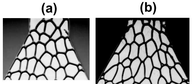
Fig. 12. Snapshots of the foam at the exit of the convergent channel, (a) for the SDS solution, (b) for the SLES/CAPB/LAc mixture. The bubbles are visibly more elongated streamwise in the latter case.
