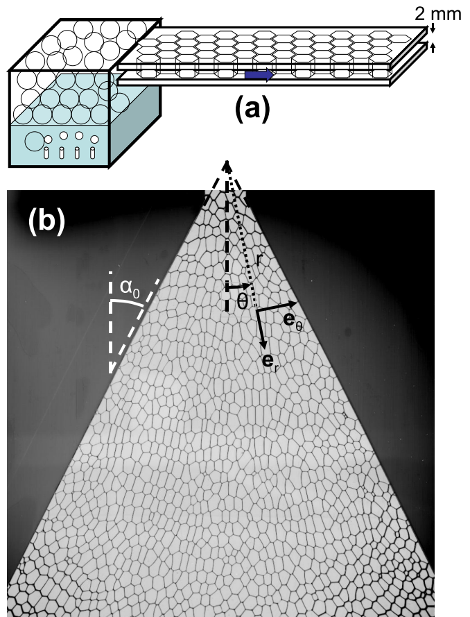
Fig. 1. (a) Sketch of the side view of the setup. For clarity, the slanted plates limiting the convergent channel have not been drawn. (b) Top view of the convergent channel, with the definition of the polar coordinates used throughout the text.
