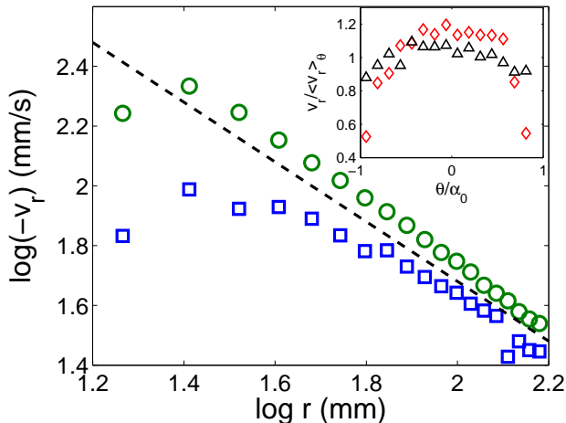
Fig. 10. Plot of \log v_r as a function of \log r , for \theta = 0 (circles) and \theta = -25^\circ (squares). The dashed line is a guide for the eye of slope -1 . Inset: plot of v_r / \langle v_r \rangle_\theta as a function of \theta , where \langle v_r \rangle_\theta is the average of the data over the angle \theta , for r = 26 mm (lozenges) and 122 mm (triangles).
