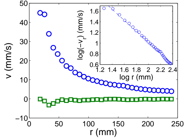
Fig. 5. Velocity components -v_r (circles) and v_\theta (squares) as a function of r , along the central axis \theta = 0 . Inset: \log(-v_r) as a function of \log r , and its best linear fit, which slope is -1.03 \pm 0.02 .
