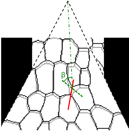
Fig. 2. Snapshot of a plastic event. Two successive skeletonised images of the foam (grey, then black) are superimposed. The link between the centres of the two bubbles which are about to lose contact is figured by the red plain line, and the link between the centres of the two bubbles that have established contact is figured by the green dashed line. The angle \beta of the appearing contact with respect to the radial direction is also figured.
