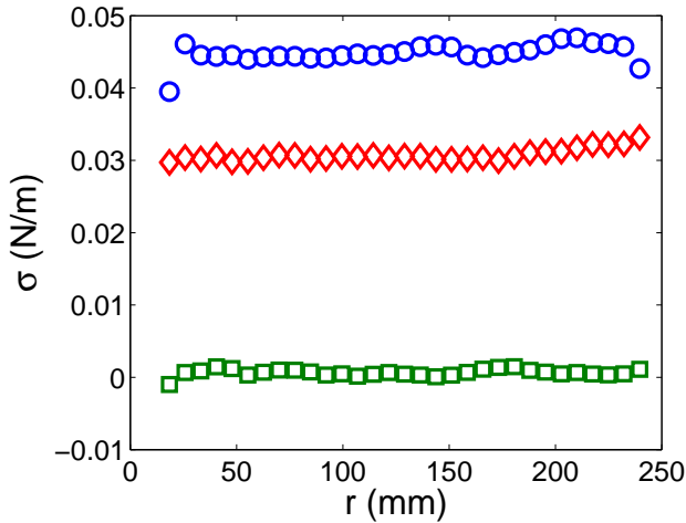
Fig. 7. Elastic stress components \sigma_{rr} (circles), \sigma_{\theta\theta} (lozenges) and \sigma_{r\theta} (squares) as a function of r , along the central axis \theta = 0 .
