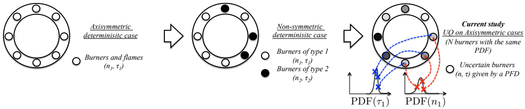
FIGURE 8. Present (right) and past (left and middle) studies on azimuthal modes. The current study introduces UQ in thermoacoustics with the same PDF for all flames. Of course, random values can be different from one burner to another. It simulates the effect of tolerance margins on burner characteristics.
