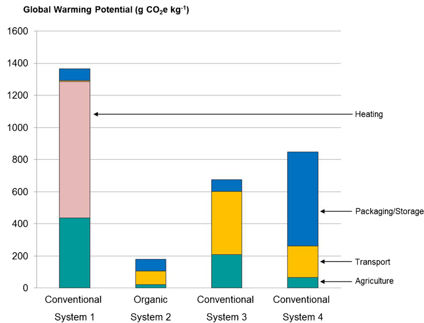
Fig. 3 Global warming potential of the key supply chains for tomatoes in absolute gram CO 2 per kilograms product at the point of sale in Austria. Total emissions are constituted by Agriculture that comprises fertilizers and pesticides, greenhouse infrastructure, soil, and greenhouse management except for Heating , which is declared separately; Packaging/Storage that includes storage, packaging, and processing stages; and Transport . A major hotspot is the Heating of Austrian Venlo
