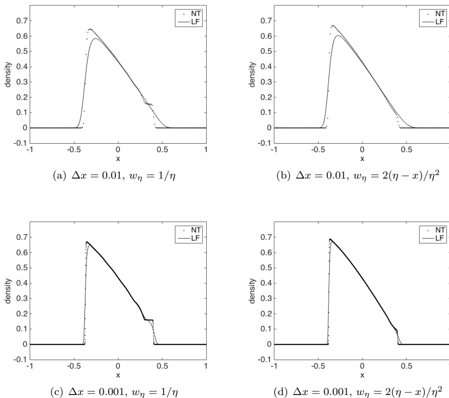
FIGURE 3. Density profiles that solve (1), (19) at time t = 0.5 computed by the Lax-Friedrichs (LF) and the Nessyahu-Tadmor (NT) schemes.
