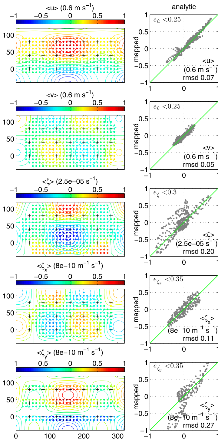
FIG. 3. 15-day mean velocity components, relative vorticity, and relative vorticity gradient components mapped from \psi, u, v with n = 0.20, T_n = 7 . (left) Analytic (contours) and mapped (dots). (right) Analytic vs mapped values for the same quantities (gray dots), with the 1:1 line shown in green. Color bars and axes have been normalized to [-1, 1] ; scale factors and units are given above the color bars and on the bottom right of each right-hand plot. The (normalized) rmsd, with the same scale as other plot quantities, are also given. The percent error variance criterion for points plotted in both left- and right-hand panels is shown in the top-left corner of each right-hand plot.
