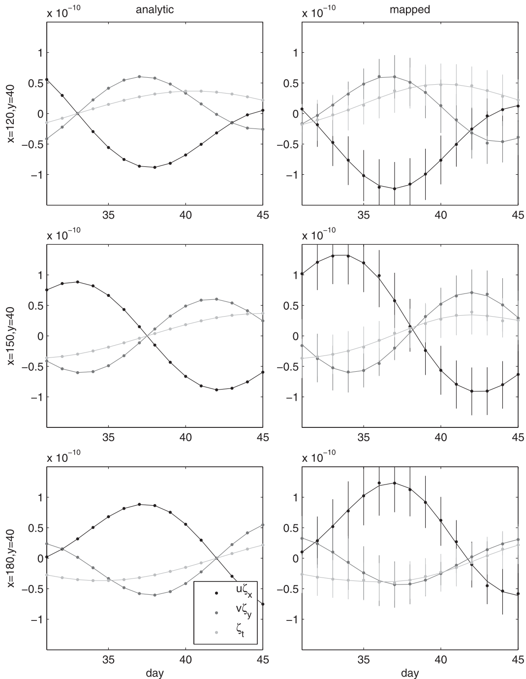
FIG. 6. As in Fig. 5, but for selected vorticity balance terms ( s^{-2} ).
