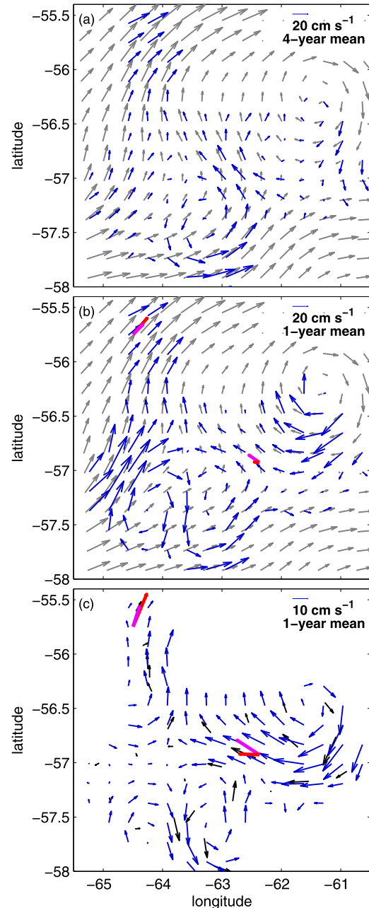
FIG. 11. (a) The 4-yr mean surface currents from cDrake (blue) and MADT (gray). (b) Means over the second M4 deployment period (10 Apr 2008–26 Mar 2009) of MADT (gray) and cDrake (blue) surface currents, with top-mooring-level moored (thick red) and cDrake (thick purple) currents at M2 (420 dbar) and M4 (520 dbar). (c) Means over the second M4 deployment period of cDrake mapped (blue) and measured (black) bottom currents, with bottom-mooring-level moored (thick red) and cDrake (thick purple) currents at M2 (2000 dbar) and M4 (2540 dbar). At the mooring sites, pressure-varying moored and cDrake currents were used. Standard errors of the mean on the cDrake currents are 1–2 \text{cm s}^{-1} . The cDrake mapped currents were subsampled from a 10-km grid to a 20-km grid for this plot, and are only shown within the good mapping region (Fig. 1).
