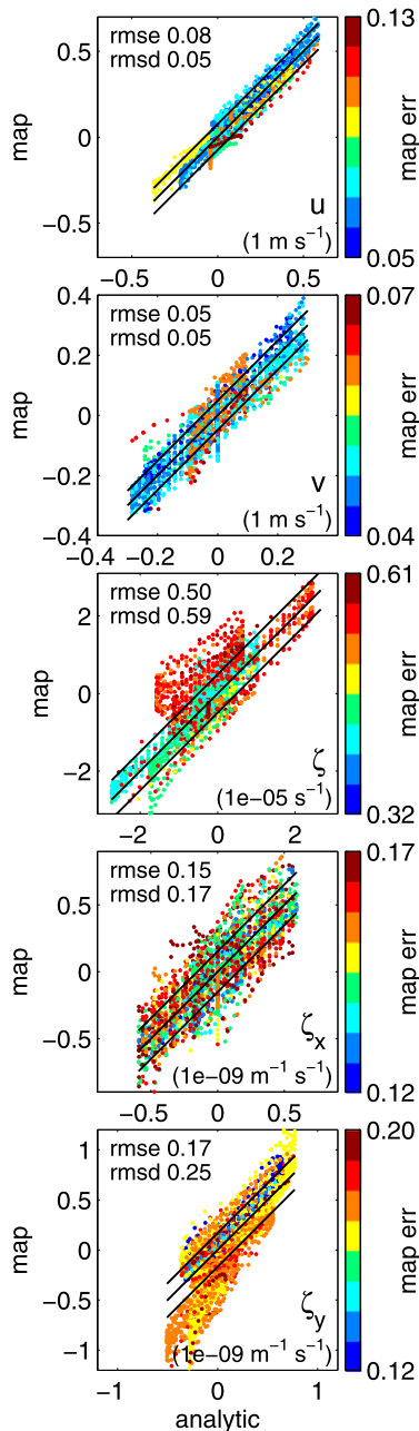
FIG. 4. Scatterplots of 15 days of daily analytic vs mapped values for (top to bottom) u , v , \zeta , \zeta_x , \zeta_y . Only points with daily percent variance mapping error e_{\theta} meeting the cutoffs given in Fig. 3 are shown. The color of each point corresponds to the mapping error \sigma_{\theta} at that point, as indicated by the color bar. The black lines are the 1:1 line and 1:1 \pm the rms of mapping error (rmse); the rmsd \delta is also given. In general, low predicted error corresponds to good agreement between mapped and analytic values, and overall rmse values describe the scatter of the mapped values about the analytic (as indicated by the black lines). Scales in the bottom-right corner of each panel apply to the axes and color bar labels as well as rmse and rmsd.
