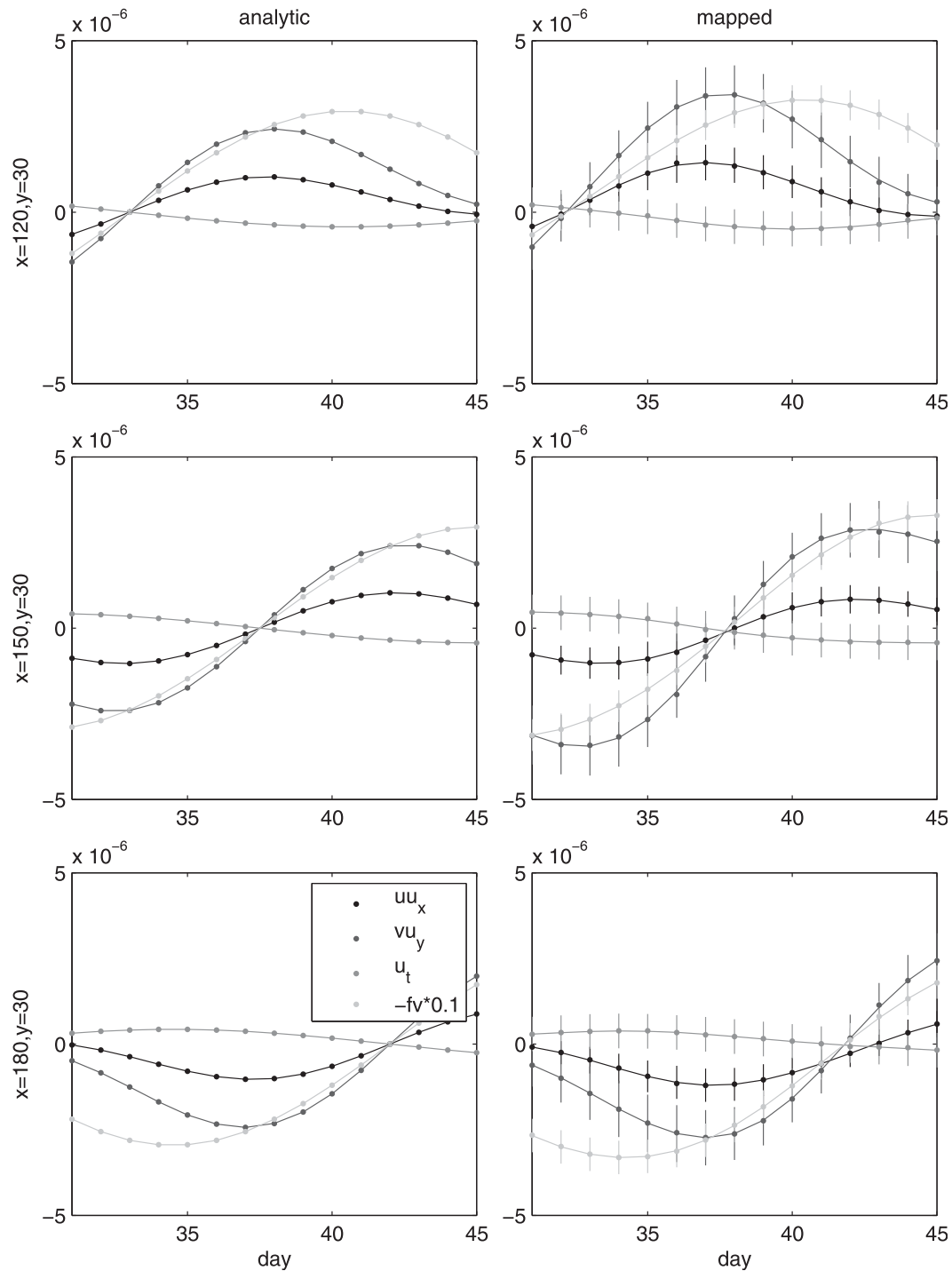
FIG. 5. (left) Analytic and (right) mapped time series of key zonal momentum balance terms ( \text{m s}^{-2} ) at three representative points in the center of the array ( x = 120, 150, 180; y = 30 ; note the central pluses in Fig. 3 are at y = 40 ). Daily data are shown by dots and data smoothed with a fourth-order Butterworth filter with a 7-day cutoff by solid lines. Vertical lines in (right) indicate standard deviation error bars on the smoothed data. Mapping was from \psi, u, v with n = 0.20, T_n = 7 (see text). The mapped tendency term, u_t , was estimated by center differencing. Note that the first-order balance is between the Coriolis term -fv and the pressure gradient term (identical by construction).
