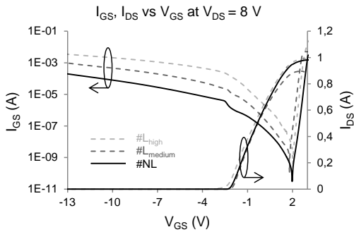
Fig. 1. Gate and drain currents versus V_{GS} for 3 DUTs: #L high , #L medium and #NL (at V_{DS} = 8 V).
