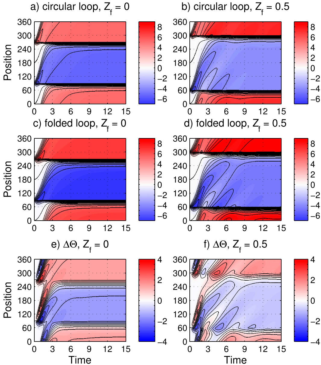
FIG. 2. Initial evolution of temperature as a function of time and position for the circular and the folded loop model. (a),(c) When source and sink are applied at Z_f = 0 , the temperature amplitudes are the same at source and sink. (b),(d) Shifting the source and sink up or down, for example, with Z_f = 0.5 , leads to an asymmetric temperature distribution. (e),(f) When the loop is folded, the temperature distribution is similar but exhibits higher amplitudes because of the significant velocity decrease, which is underlined by the temperature difference \Delta\Theta = \Theta(\text{full}) - \Theta(\text{folded}) . Contour lines are placed at intervals of 1 in (a)–(d) or 0.5 in (e) and (f).
