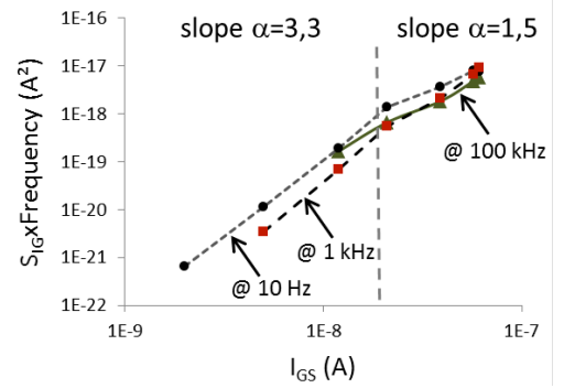
Fig. 8. S_{IG}\times\text{frequency} versus I_{GS} (at 1 Hz, 1 kHz, 100 kHz).
