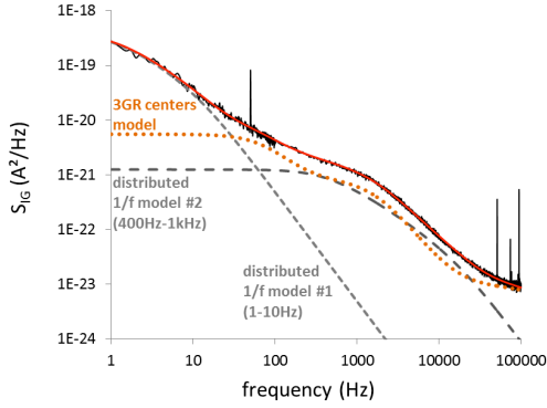
Fig. 6. Gate current spectral density S_{IG} versus frequency (open drain, V_{GS}=-1\text{V} ), and associated model based on 2 distributed 1/f models (1-10Hz and 400-1000Hz) [6] and 3 GR centers (80Hz, 1.7kHz, and above 200kHz).
