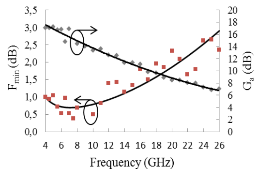
Fig. 1. Minimum noise figure F_{\min} and Associated Gain G_a versus frequency for an InAlN/GaN MOS-HEMT ( 0.15 \times 2 \times 75 \mu\text{m}^2 , V_{DS}=5\text{V} and V_{GS}=-1\text{V} ).
