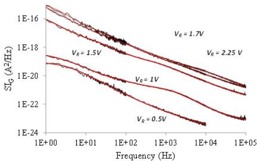
Fig. 7. Gate current spectral density S_{IG} versus frequency (open drain), for variable reverse gate bias V_R .
