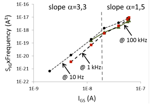
Fig. 8. S_{IG}\times\text{frequency} versus I_{GS} (at 1 Hz, 1 kHz, 100 kHz).
