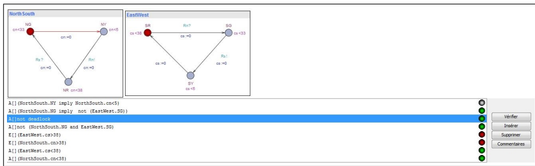
Figure 10: Uppaal environment
