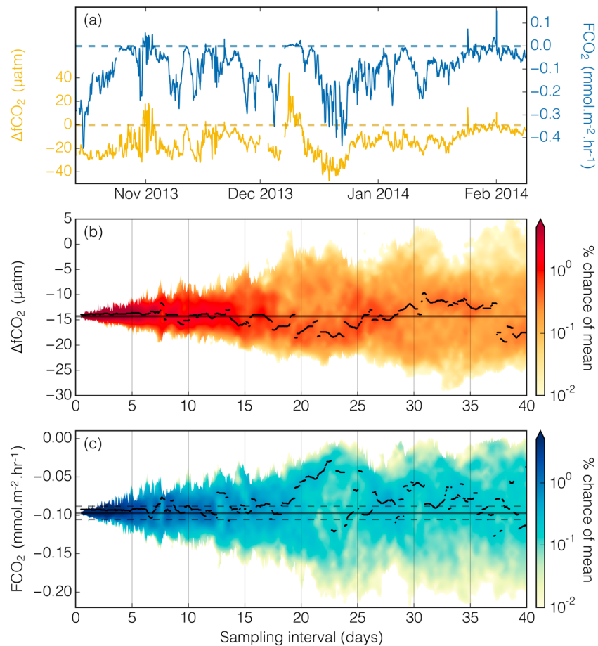
Figure 2. (a) 4 month time series of observed \Delta f\text{CO}_2 ( \mu\text{atm} ) and derived fluxes \text{FCO}_2 ( \text{mmol}\cdot\text{C}\cdot\text{m}^{-2}\cdot\text{h}^{-1} ) from the SOSCEX II sampling location in the SAZ. It shows the strong intraseasonal modes and highlights important differences in the intraseasonal timing between the two variables. (b and c) The sensitivity of the sampling means of \Delta f\text{CO}_2 (Figure 2b) and \text{FCO}_2 (Figure 2c) to the sampling interval (period). The widening ranges indicate how, in systems characterized by strong intraseasonal variability, the uncertainty in the mean seasonal \Delta f\text{CO}_2 and \text{FCO}_2 increase as the sampling frequency decreases. The dashed lines represent the 10% uncertainty threshold on either side of the hourly data mean, and the broken solid line depicts the variability of the mode. It shows (right-hand scale) that the probability of achieving the accurate hourly sampling mean falls rapidly with increasing sampling period to < 1\% above a 10 day period.
