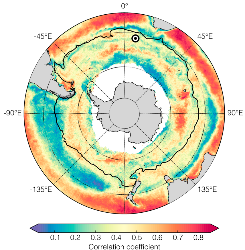
Figure 1. The sampling location for SOSCEX II (black-white dot) was in a region of intraseasonal dynamics in the Sub-Antarctic Zone south of Africa and that these characteristics extend over at least 30% of the area of the Southern Ocean. The mean positions of the Sub-Tropical Front (STF) and the Polar Front (PF) are depicted over the spatial characteristics of the correlation of the seasonal cycle (1998–2007) with the decadal mean of the seasonal cycle of satellite chlorophyll a . Areas of low correlation ( r^2 < 0.4 : low seasonal cycle reproducibility) are dominated by intraseasonal dynamics and a high correlation coefficient ( r^2 > 0.4 : high seasonal cycle reproducibility) are characterized by a seasonal cycle reproducible interannually.
