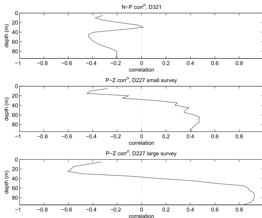
Figure 8. Variation of correlation with depth (top) between nitrate and phytoplankton from cruise D321 and between phytoplankton and zooplankton from cruise D227 for (middle) small and (bottom) large surveys. Note that the vertical resolution is greater than the 10 m interval (25–35 m) used elsewhere.
