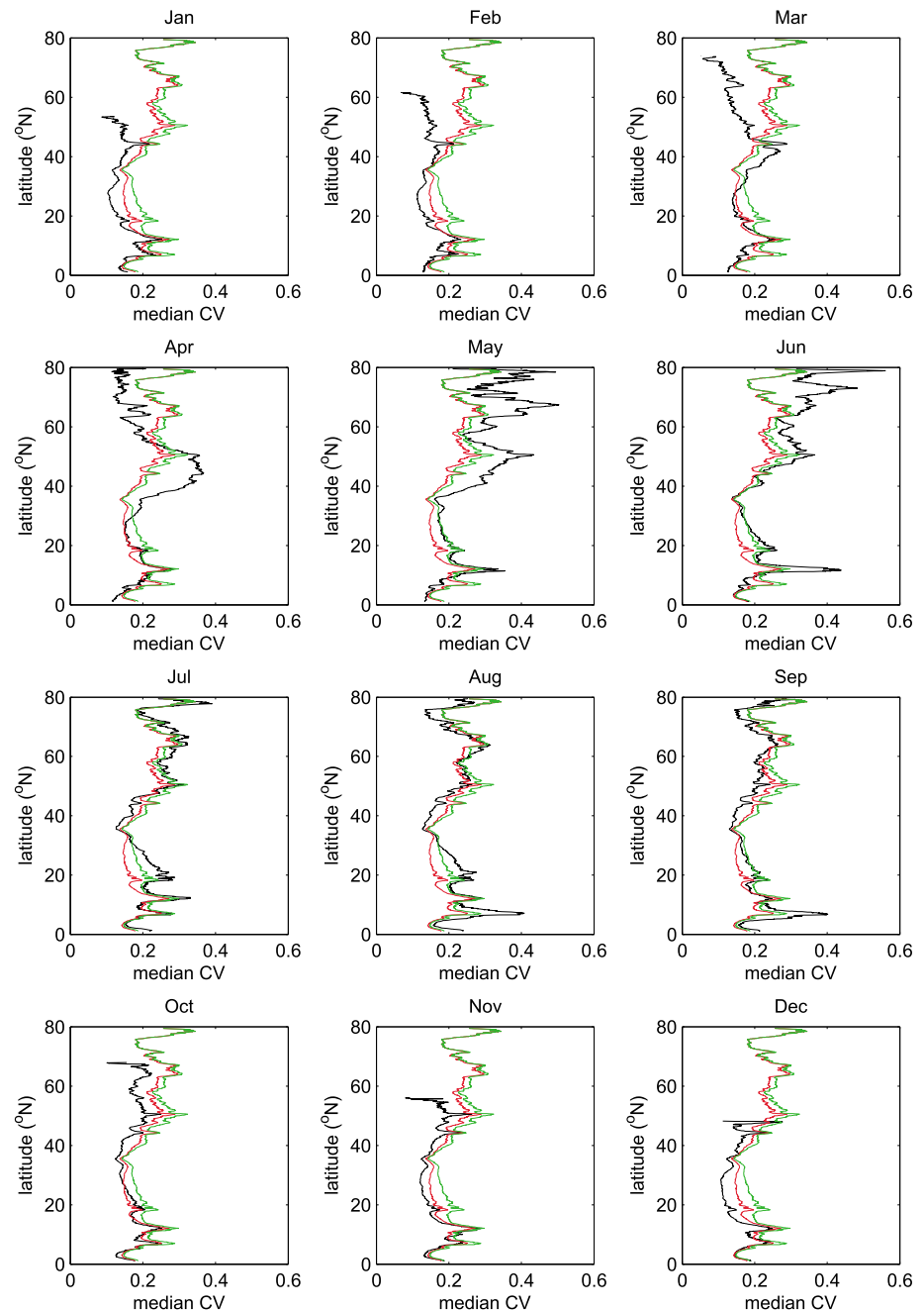
Figure 6. Median coefficient of variation for chlorophyll a at each latitude and each month (black line). The median coefficient using data from the whole year is also shown in each panel (red line). The green line shows estimates using data restricted to March to September. Data are from the MODIS Aqua satellite—see Acknowledgements.
