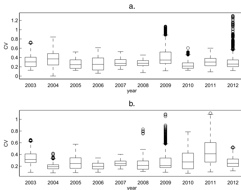
Figure 7. Box plot of coefficient of variation (CV) in 130 km \times 130 km region centered on (a) 59°N, 19°W for cruise D321 and (b) 47.5°N, 18°W for cruise D227 for the years 2003–2012. For each year, the box plot uses all estimates from July to August for D321 and April and May for D227, to match the period of the cruises. The centerline is the median; the box top and bottom are the 75% and 25% quartile limits; the whiskers denote the extent of 1.5 \times IQR on either side of the box, where IQR is the interquartile range; and points outside the whiskers are marked individually as outliers. Each box plot uses 5103 and 5832 data points for D321 and D227, respectively.
