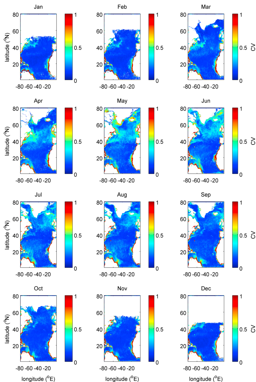
Figure 5. Monthly climatology of median coefficient of variation for chlorophyll a for the years 2003–2012. Each pixel value is calculated using data in a box of side 1.13° centered upon it—see section 2.2. Data are from the MODIS Aqua satellite—see Acknowledgements.
