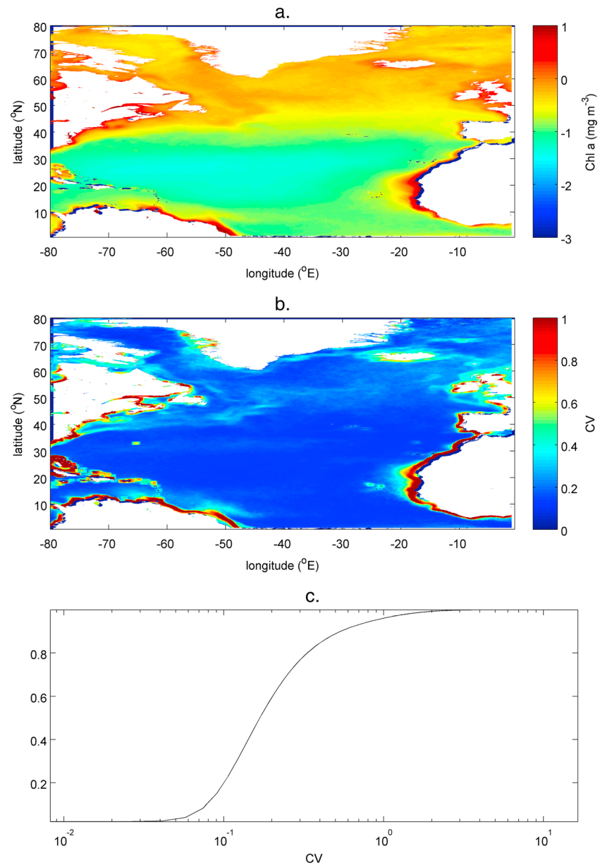
Figure 4. For the years 2003–2012: (a) average daily phytoplankton abundance ( \text{Chl } a \text{ mg m}^{-3} ), (b) median coefficient of variation for phytoplankton abundance in an area 1.13^\circ \times 1.13^\circ centered on each pixel, and (c) cumulative distribution for CV including estimates every 8 days for each pixel for this period. Data are from the MODIS Aqua satellite—see Acknowledgments.
