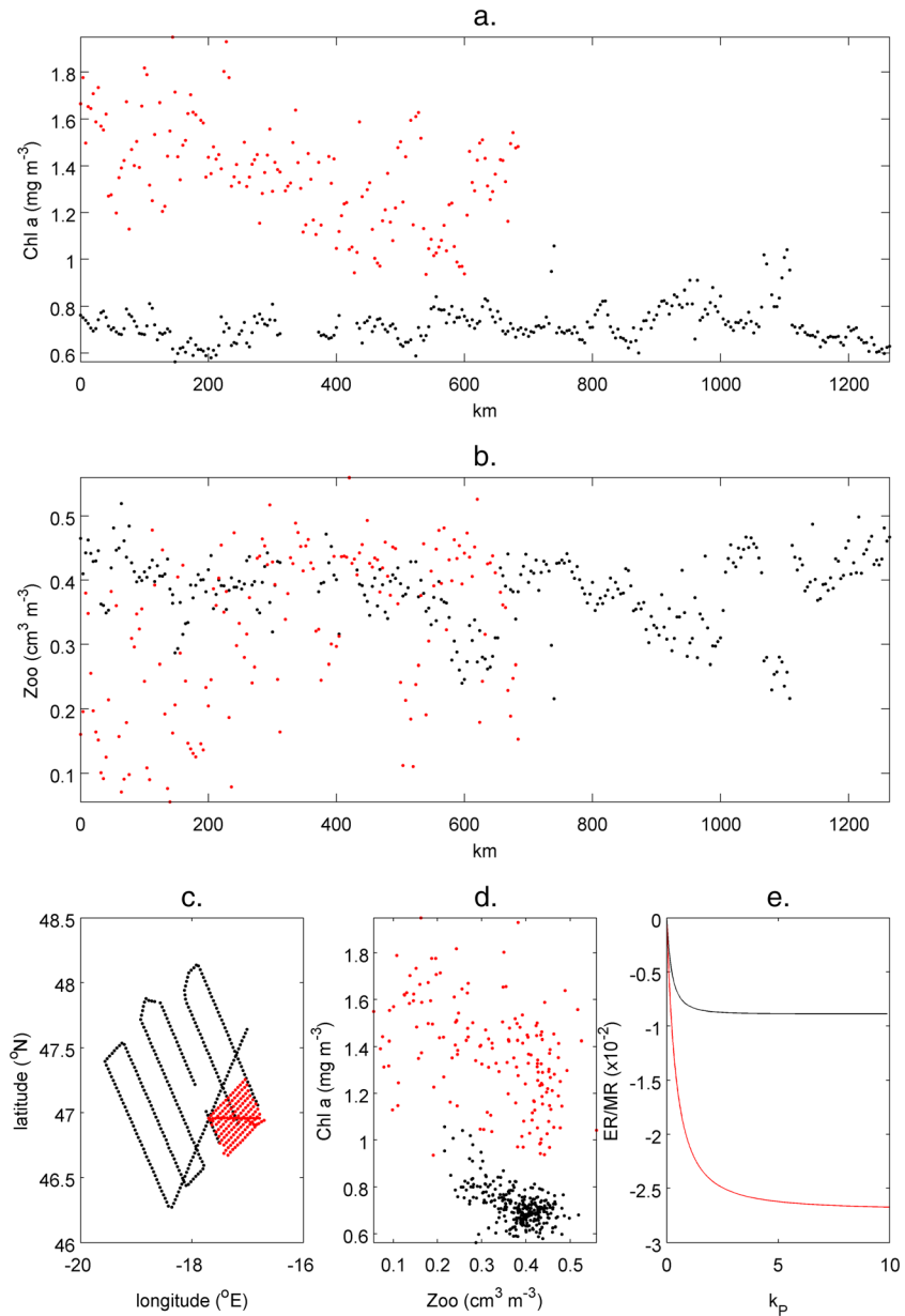
Figure 3. Analysis of relative magnitudes of eddy and mean reaction terms for zooplankton grazing (equation (2)) using data from cruise D227. Results from analyzing two spatial surveys are shown, the first (red) from 1 to 3 May 1997 and the second (black) from 10 to 13 May 1997: (a) Chl a data shown against distance traveled (km), (b) zooplankton abundance data shown against distance, (c) positions of observations, (d) scatterplot of Chl a and zooplankton observations, and (e) relative size of eddy reaction (ER) and mean reaction (MR) terms for a range of values for phytoplankton half saturation, k_p .
