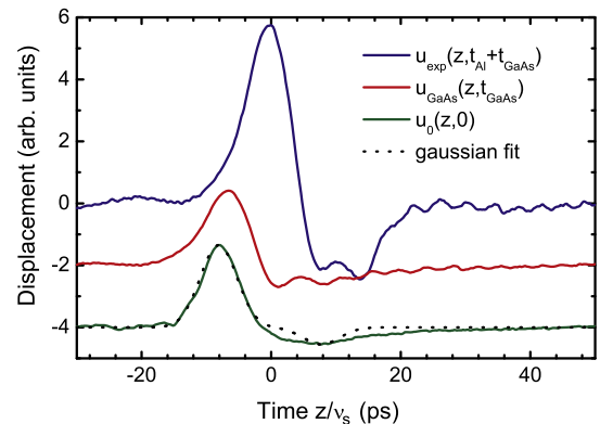
Fig. 4. Displacement pulses u_{exp}(z, r=0, t_{Al} + t_{GaAs}) measured at sample surface (blue), u_{GaAs}(z, r=0, t_{GaAs}) retrieved at Al/GaAs interface (red) and u_0(z, r=0, t=0) before propagation through the GaAs substrate (green). Dotted line: displacement of Gaussian initial pulse. (For interpretation of the references to colour in this figure legend, the reader is referred to the web version of this article.)
