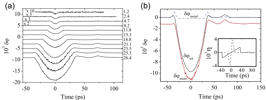
Fig. 8. (a) Phase signal versus z/v_s , obtained by probing the sapphire crystal opposite the pump spot, as a function of pump fluence. Data have been published in Ref. [19]. (b) Calculation of the bulk phase signal contribution \delta\phi_{metal} (dashed line) to the total phase signal \delta\phi_{tot} , and comparison to the measured signal \delta\phi for a fluence of 26.4 \text{ mJ/cm}^2 . The measured signal is displaced by 10^{-3} to enhance visibility. Inset shows the initial wave shape (dashed line), and the wave shape after propagation through 126 \mu\text{m} of sapphire (solid line), obtained from a numerical calculation.
