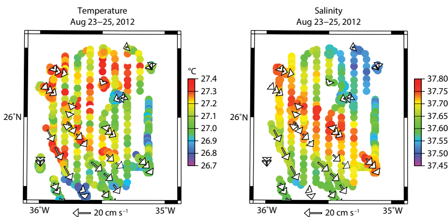
FIGURE 4. STRASSE mesoscale SST on left panel, and SSS on right panel, August 23–25, 2012. Daily variations were removed as well as possible longer trends due to cooling and mixed-layer depth deepening. The arrows correspond to daily Surface Velocity Program drifter trajectories. Estimates of Ekman drifts have not been removed, as mixed-layer depth is rather shallow during this period.
