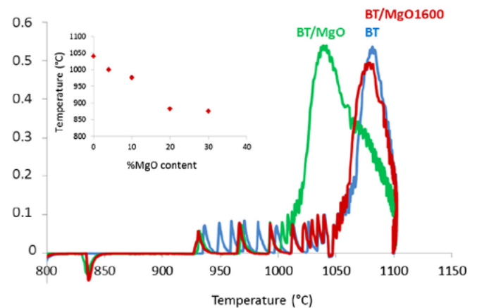
Fig. 3. Speed of shrinkage recorded during SPS sintering of BT (blue), BT/MgO (green) and BT/MgO1600 (red) composites versus temperature. Inset: onset of displacement for BT/MgO composites versus the MgO content. (For interpretation of the references to color in this figure legend, the reader is referred to the web version of this article.)
