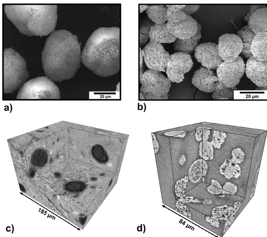
Fig. 1. MgO granules observed by SEM and XCMT. (a) SEM image of MgO granules sorted at \approx 30 \mu\text{m} diameter. (b) SEM image of MgO granules annealed at 1600^\circ\text{C} . (c) Multiple cross-section images of the initial microstructure of BT-MgO composite obtained by XCMT. MgO are in dark gray levels and the BT matrix is in light gray. (d) MgO granules annealed at 1600^\circ\text{C} . Particles were loaded into glass capillary tubes.
