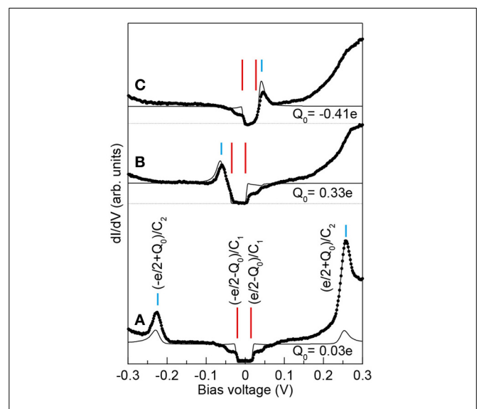
FIGURE 6 | Manipulation of the residual charge Q_0 . dI/dV spectra measured on the same island with 7.9 nm side, showing features related to both, C_1 and C_2 , with varying Q_0 , and corresponding simulations. The residual charge ( Q_0 ) of the island is changed by a bias voltage pulse (duration: 50 \mu\text{s} , current: 1 \text{ nA} ). Parameters of the simulation: C_1 = 3.8 \text{ aF} , C_2 = 0.335 \text{ aF} , R_1 = 25 \text{ M}\Omega , R_2 = 2300 \text{ M}\Omega ; (A): Q_0 = 0.03 e , (B): Q_0 = 0.33 e , (C): Q_0 = -0.41 e .
