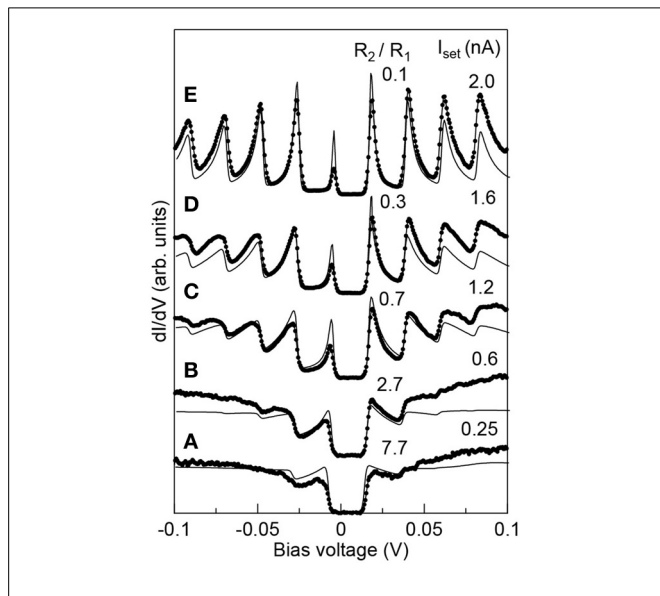
FIGURE 4 | Evolution from Coulomb blockade to Coulomb staircase: experimental STS data acquired on a Pb island with 14 nm side ( A_{\text{island}} \approx 85 \text{ nm}^2 ) (dots) and simulation (black line) based on the orthodox theory. The spectra are offset for clarity. Parameters of the simulation: R_1 = 39 \text{ M}\Omega , C_1 = 7.46 \text{ aF} , and C_2 = 0.7 \text{ aF} ; (A): R_2 = 300 \text{ M}\Omega and Q_0 = -0.15 e , (B): R_2 = 105 \text{ M}\Omega and Q_0 = -0.2 e , (C): R_2 = 26 \text{ M}\Omega and Q_0 = -0.26 e , (D): R_2 = 13 \text{ M}\Omega and Q_0 = -0.26 e , (E): R_2 = 4.5 \text{ M}\Omega and Q_0 = -0.28 e .
