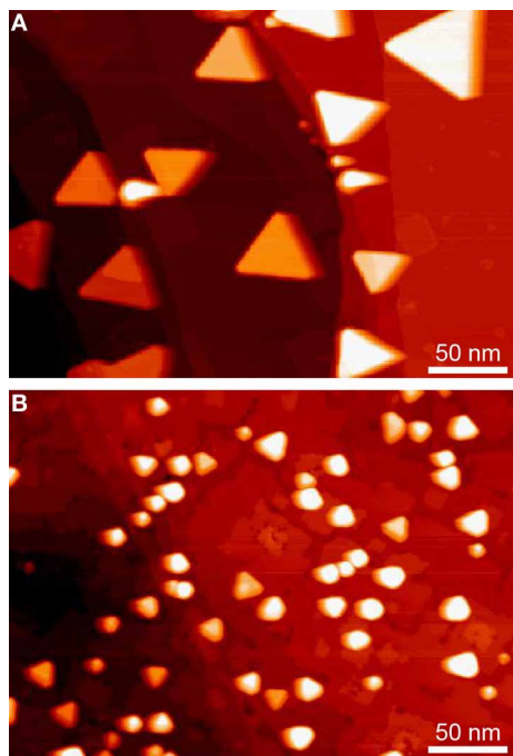
FIGURE 2 | STM topographies acquired on two different samples with Pb islands grown on NaCl/Ag(111). Pb islands are visible in both images, most of them with triangular shape and a few with rounded shape. The smaller island size in (B) as compared to (A) is obtained on a NaCl film exhibiting more defects. (A): +1 V, 20 pA; (B): +4 V, 20 pA.
