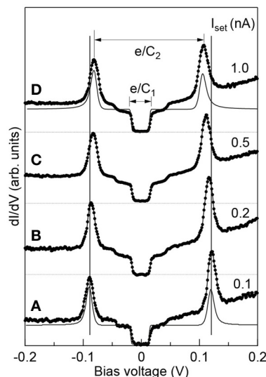
FIGURE 5 | Spectra (A to D): increase of the tip-island capacitance C_2 with decreasing tip-island distance (increasing tunnel current). The spectra, offset for clarity as dI/dV(0V) = 0 , have been acquired on a Pb island of 14 nm side. Parameters of the simulation, performed for spectra (A) and (D) curve: C_1 = 5.0 \text{ aF} , C_2 = 0.77 \text{ aF} , R_1 = 5 \text{ M}\Omega , R_2 = 1700 \text{ M}\Omega , Q_0 = 0.062 e ; (D) curve: C_1 = 5.0 \text{ aF} , C_2 = 0.86 \text{ aF} , R_1 = 5 \text{ M}\Omega , R_2 = 145 \text{ M}\Omega , Q_0 = 0.07 e .
