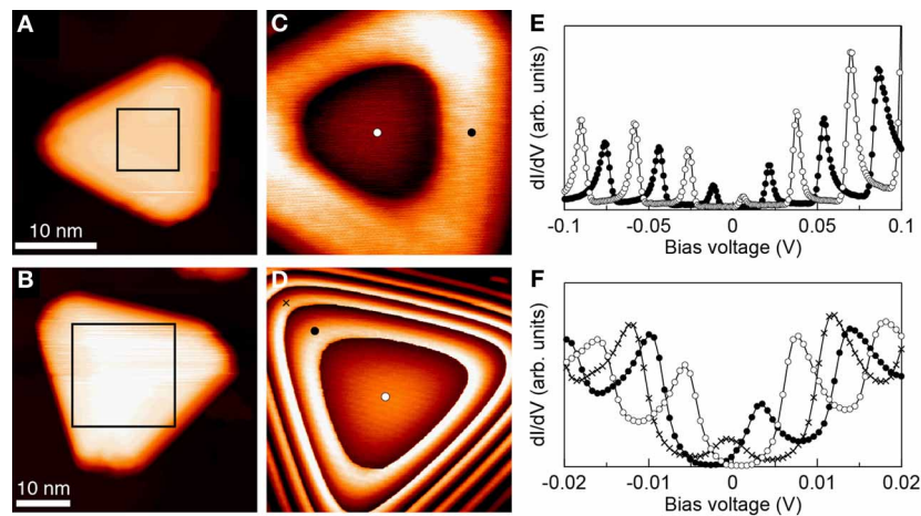
FIGURE 7 | (A,B) Topographic images of Pb islands on NaCl; (A) : -1 V, 20 pA; (B) : 2.5 V, 20 pA; (C,D) Close-up view; (C) : -0.15 V, 200 pA; (D) : -0.01 V, 20 pA; (E,F) dI/dV spectra acquired on the locations represented by the corresponding symbol, showing different values of Q_0 (see text).
