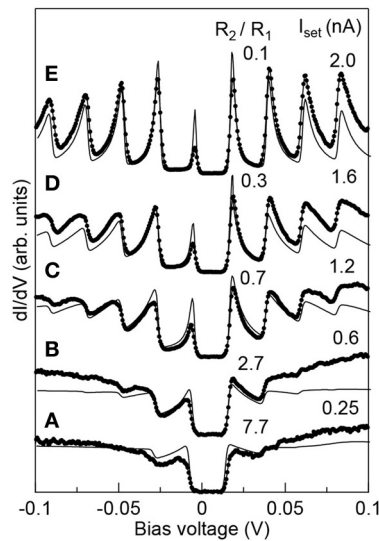
FIGURE 4 | Evolution from Coulomb blockade to Coulomb staircase: experimental STS data acquired on a Pb island with 14 nm side ( A_{\text{island}} \approx 85 \text{ nm}^2 ) (dots) and simulation (black line) based on the orthodox theory. The spectra are offset for clarity. Parameters of the simulation: R_1 = 39 \text{ M}\Omega , C_1 = 7.46 \text{ aF} , and C_2 = 0.7 \text{ aF} ; (A): R_2 = 300 \text{ M}\Omega and Q_0 = -0.15 e , (B): R_2 = 105 \text{ M}\Omega and Q_0 = -0.2 e , (C): R_2 = 26 \text{ M}\Omega and Q_0 = -0.26 e , (D): R_2 = 13 \text{ M}\Omega and Q_0 = -0.26 e , (E): R_2 = 4.5 \text{ M}\Omega and Q_0 = -0.28 e .
