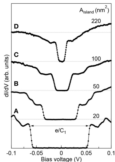
FIGURE 3 | dI/dV spectra labeled (A to D) acquired on four Pb islands with different area A_{\text{island}} . A Coulomb gap of decreasing size is visible in going from spectrum (A to D) reflecting a Coulomb blockade process.
