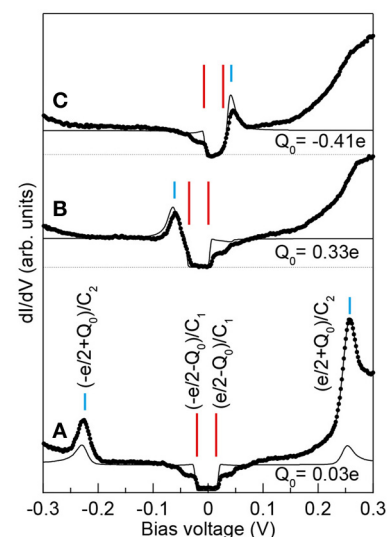
FIGURE 6 | Manipulation of the residual charge Q_0 . dI/dV spectra measured on the same island with 7.9 nm side, showing features related to both, C_1 and C_2 , with varying Q_0 , and corresponding simulations. The residual charge ( Q_0 ) of the island is changed by a bias voltage pulse (duration: 50 \mu\text{s} , current: 1 \text{ nA} ). Parameters of the simulation: C_1 = 3.8 \text{ aF} , C_2 = 0.335 \text{ aF} , R_1 = 25 \text{ M}\Omega , R_2 = 2300 \text{ M}\Omega ; (A): Q_0 = 0.03 e , (B): Q_0 = 0.33 e , (C): Q_0 = -0.41 e .
