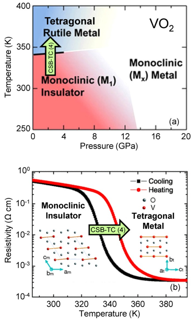
Figure 5 : (a) Temperature-pressure phase diagram of \text{VO}_2 . Adapted with permission from Ref. [54], Copyright 2014, American Institute of Physics. (b) Resistivity vs. temperature at the “type 4” insulator to metal transition (IMT) in \text{VO}_2 . This IMT is associated with a Crystallographic Symmetry Breaking between the monoclinic low- T and the tetragonal high- T phases. Reproduced with permission from Ref. [55], Copyright 2013, American Physical Society.
