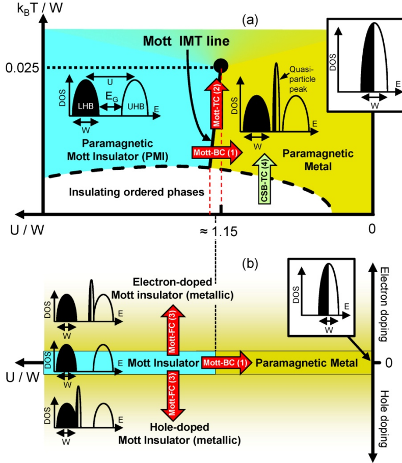
Figure 1 : (a) Schematic phase diagram of two- and three-dimensional half-filled compounds undergoing a Mott insulator to metal transition, displayed as k_B T / W vs. U / W . T , U and W are the temperature, the Hubbard electron-electron repulsion term and the bandwidth, respectively. Typical electronic Density of States (DOS) are displayed in relevant regions of the phase diagram : in absence of electron correlation ( U / W = 0 ), in the correlated metal domain slightly below U / W = 1.15 and in the Mott insulating state for U / W > 1.15 . (b) Diagram of doped Mott insulators, represented as electron and hole doping away from half-filling vs. correlation strength U / W , for intermediate temperature T_{ordered\ phase} < T < T_{endpoint} shown in part (a).
