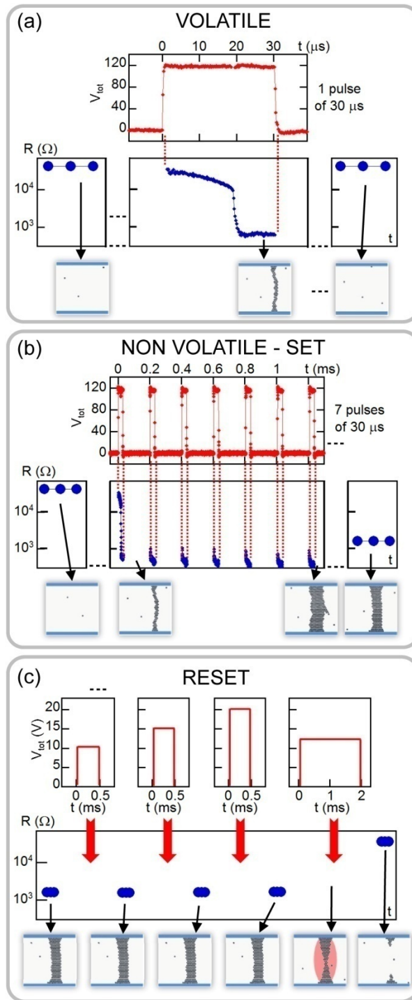
Figure 10 : Resistance variation of a GaV 4 S 8 crystal, before, during and after applying (a) 1 pulse of 30 \mu\text{s} / 120V, and (b) a train of 7 pulses of 30 \mu\text{s} / 120V every 200 \mu\text{s} leading to SET non-volatile transition. As expected, the resistance drop during the first pulse shown in (b) is similar to the one occurring during the single pulse in (a). Noteworthy the resistance does not go back to a high resistance state between and during the subsequent pulses. The resistances before and after the application of the (series of) pulses are measured at low bias and are displayed as blue circles. (c) Pulse duration impact on the RESET transition in a GaV 4 S 8 crystal. 500 \mu\text{s} pulses in the 10-20 V range do not affect resistance level, whereas a 2 ms / 12V pulse induces the RESET transition. The additional sketches illustrate the evolution of the conductive filament through the application of successive pulses.
