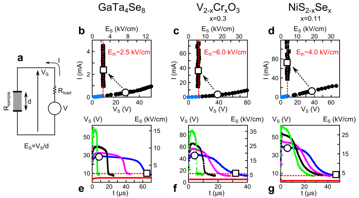
Figure 8. Panel a shows the schematics of the experimental setup. Universal dielectric breakdown I - V characteristics (top panels b , c , d ) and time dependence of the sample voltage V_S(t) (bottom panels e , f , g ) are displayed for three different types of narrow gap Mott insulators. Blue dots correspond to the region below E_{th} , where no breakdown is observed. Black symbols correspond to the I - V characteristic in the resistive switching region, above E_{th} . The black dots show the initial I - V , before the breakdown, and the black squares indicate the final state. The open symbols highlight a particular breakdown transition for easier visualization. Measurements on \text{GaTa}_4\text{Se}_8 were performed at 77 K [8], on \text{V}_{2-x}\text{Cr}_x\text{O}_3 ( x=0.3 ) at 164 K and on \text{NiS}_{2-x}\text{Se}_x ( x=0.11 ) at 4 K. Reproduced with permission from Ref. [108], Copyright 2013, WILEY-VCH Verlag GmbH & Co.
