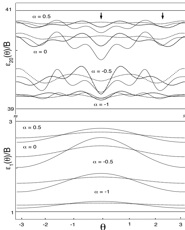
Figure 1: The eigenvalues of H_{\alpha, l}(\theta) in the units of B . (Top) n = 20 , B = 4 (full line), B = 6 (full dotted line) and B = 8 (dotted line). (Bottom) n = 1 , B = 10 (full line) and B = 15 (dotted line). The thick lines represent the Landau levels.
