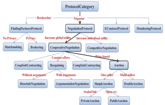
Fig. 6. Protocol Taxonomy
