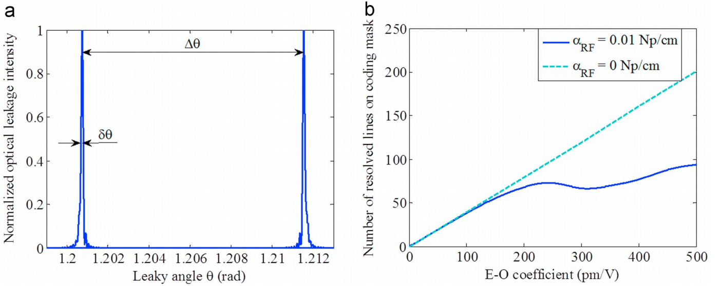
Fig. 9: Simulation results obtained with Eq. (8) with L=3 cm, \alpha_{\text{opt}}=0.345 Np/cm, \alpha_{\text{RF}}=0.01 Np/cm (after RF attenuation compensation), \alpha_{\text{leak}}=0.1 Np/cm, \Gamma=100\% , V_{\text{RF}}=\pm 20 V and gap between strips G_0=4.2 \mu\text{m} . (a) Leaky intensity peaks for applied voltages V=-20 and +20 V and r_{\text{eo}}=350 pm/V. (b) Number of resolved lines on the coding mask versus E-O coefficient.
