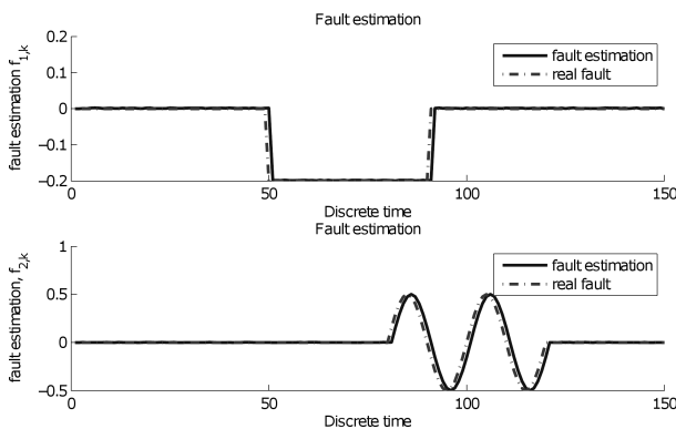
Fig. 5. Faults and their estimates (by P. Witczak)
