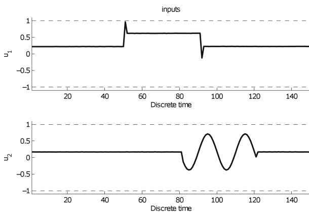
Fig. 6. Respective control inputs u_1, u_2 (by P. Witczak)
