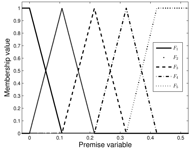
Fig. 3. Fuzzy sets used in the Takagi-Sugeno model (by P. Witczak)
