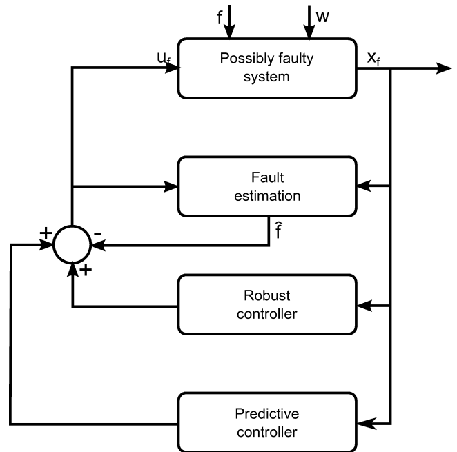
Fig. 1. Proposed robust predictive FTC scheme outline (by P. Witczak)
