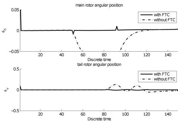
Fig. 4. Selected states of the system with with and without FTC (by P. Witczak)
