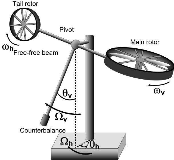
Fig. 2. Components of the twin-rotor MIMO system (by P. Witczak)
