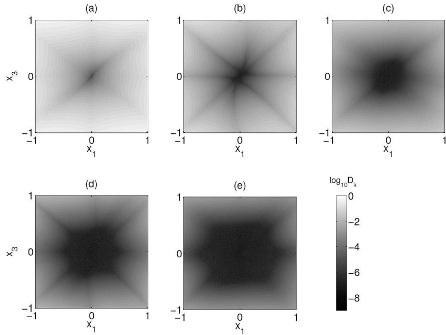
Figure 1: The simplicity defect of the controlled map T_k(F_2) 4.38. Plot of \log_{10} D_k , where D_k = \|A_k^T J A_k - J\| and A_k is the Jacobian of the k -order controlled map T_k(F_2) given by 4.38, for 16000 uniformly distributed values in the square (x_1, x_3) \in [-1, 1] \times [-1, 1] , x_2 = x_4 = 0 , for (a) k = 1 , (b) k = 2 , (c) k = 3 , (d) k = 4 and (e) k = 5 . The percentage of orbits with \log_{10} D_k < -4 is 0.5%, 11%, 28%, 53% and 73% for k = 1, 2, 3, 4 and 5 respectively. The gray scale corresponds to the value of \log_{10} D_k : the darker the color, the smaller the value of \log_{10} D_k is, and hence the closer the map is to a symplectic one.
