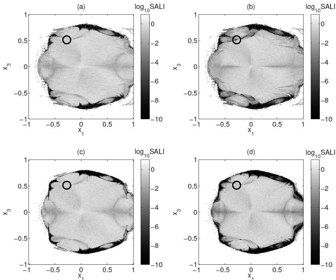
Figure 4: Stability analysis in the (x_1, x_3) plane. 16000 uniformly distributed initial conditions in the square (x_1, x_3) \in [-1, 1] \times [-1, 1] , x_2(0) = x_4(0) = 0 are integrated using the T_3(F_2) ((a) and (b)), and the T_4(F_2) controlled map ((c) and (d)), up to n = 10^4 ((a) and (c)) and n = 10^5 iterations ((b) and (d)). The gray scale represents the value of \log_{10}SALI for each orbit at the end of the integration time. The lighter the color the more stable is the orbit, while white color denotes that an orbit escaped before the total number of iterations was reached. The black circle indicate the initial condition of the orbit studied in Fig. 5.
