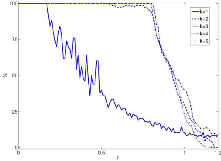
Figure 3: Percentages of non-escaping orbits for the controlled map T_k(F_2) 4.38 as a function of the distance from the origin in the physical space (x_1, x_3) . We iterate initial conditions in a circle of radius r centred at the origin of plane (x_1, x_3) , with x_2(0) = x_4(0) = 0 , and compute the percentages of non-escaping orbits during n = 10^5 iterations, for the controlled map T_k(F_2) with k = 1, 2, 3, 4, 5 , as a function of r .
