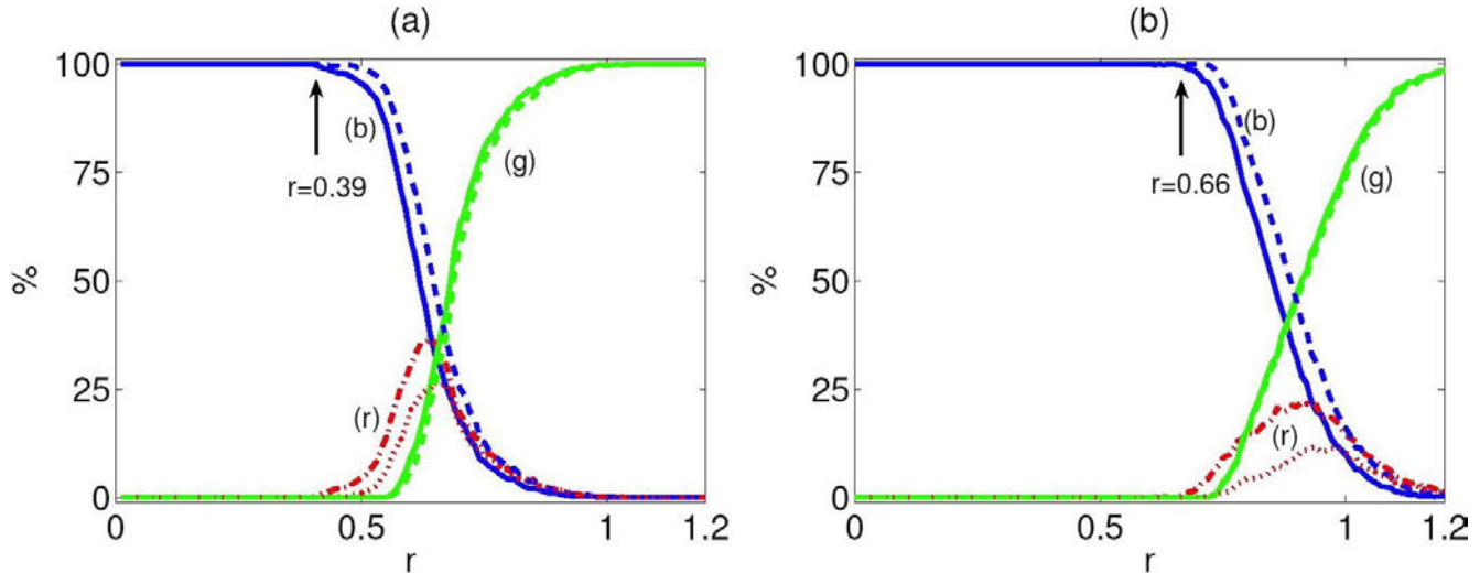
Figure 6: (Color online) Dynamical aperture of the (a) original map (2.1) and (b) the T_4(F_2) controlled map (4.38). The percentages of regular [(b) blue curves], escaping [(g) green curves] and chaotic [(r) red curves] orbits after n = 10^4 (dashed curves) and n = 10^5 iterations (solid curves) for initial conditions in a 4D sphere centred at the origin x_1 = x_2 = x_3 = x_4 = 0 , as a function of the sphere radius r . Each point corresponds the average value over 5000 initial conditions. The largest radius at which the percentage of regular orbits is still 100%, is marked by an arrow in each panel.
