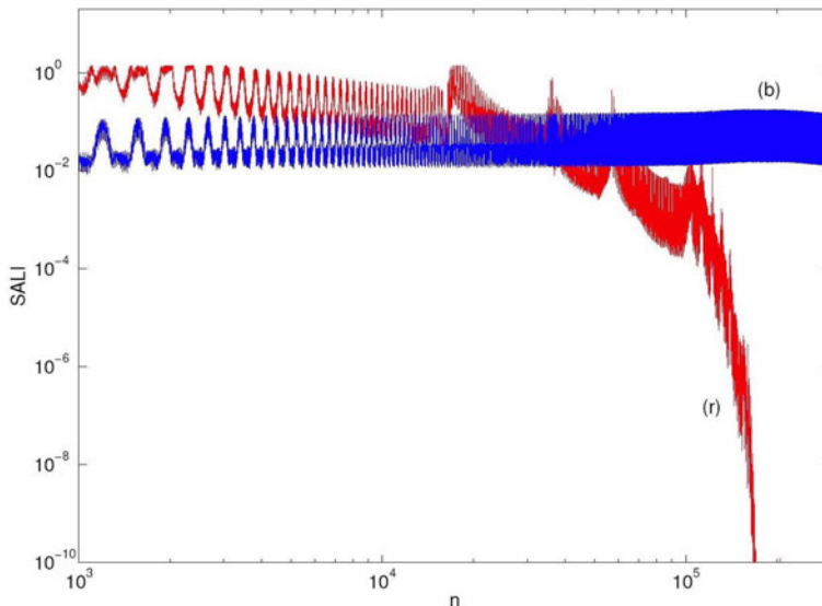
Figure 5: (Color online) Dynamics of two orbits with the same initial conditions for the 3 rd and 4 th order controlled maps. Time evolution of the SALI for the orbit with initial conditions \vec{x}(0) = (-0.50, 0, -0.65, 0)^T (see Fig. 4), using the T_3(F_2) [(r) red curve] and the T_4(F_2) controlled map [(b) blue curve].
