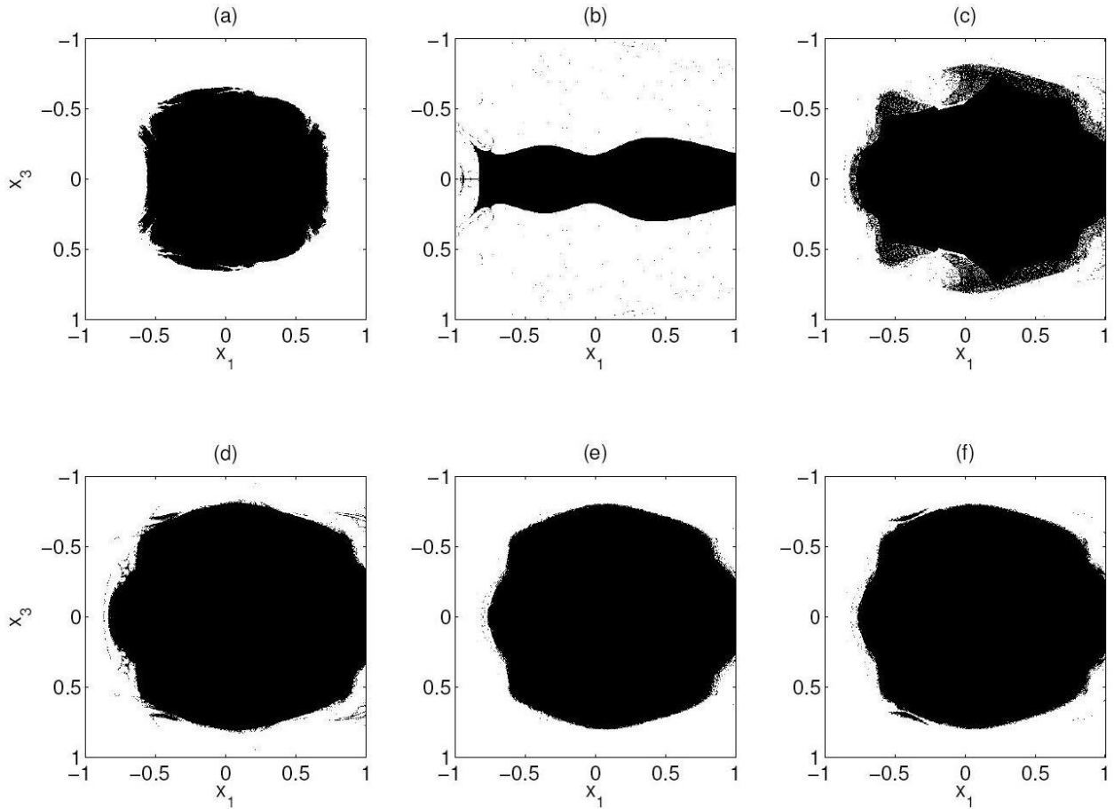
Figure 2: Non-escaping regions of controlled map T_k(F_2) as a function of the truncation order k . 16000 uniformly distributed initial conditions in the square (x_1, x_3) \in [-1, 1] \times [-1, 1] , x_2(0) = x_4(0) = 0 are iterated up to n = 10^5 using (a) the uncontrolled map 2.1 and (b)–(f) the k = 1 to k = 5 order controlled map T_k(F_2) 4.38, respectively. Initial conditions corresponding to non-escaping orbits up to n = 10^5 are coloured in black, while escaping orbits are colored in white.
