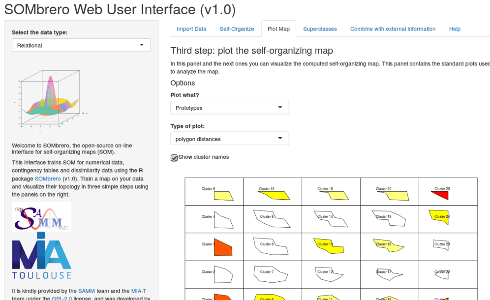
FIGURE 1. Screenshot of the SOMbrero web user interface
