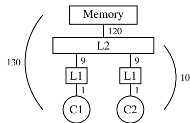
Fig. 6. Architecture of the memory
