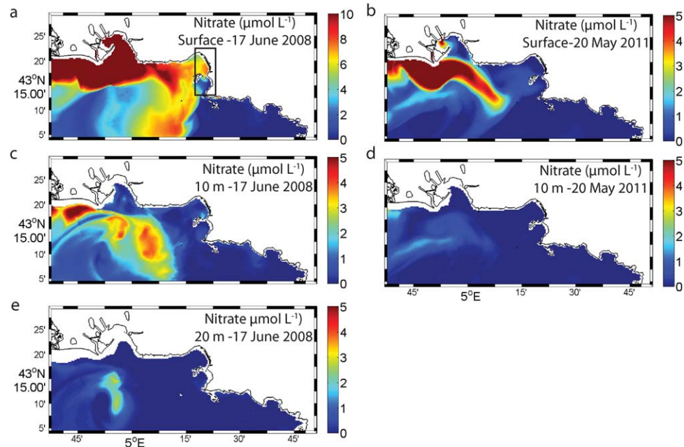
Figure 8. Modeled nitrate concentrations ( \mu\text{mol L}^{-1} ) on 17 June 2008 (a) at the surface (5 m average), (c) at 10 m (1 m average), (e) at 20 m (1 m average) and on 20 May 2011 (b) at the surface (5 m average) and (d) at 10 m (1 m average). The 20 m depth on 20 May 2011 is not shown as there is no visible trace of the plume.
