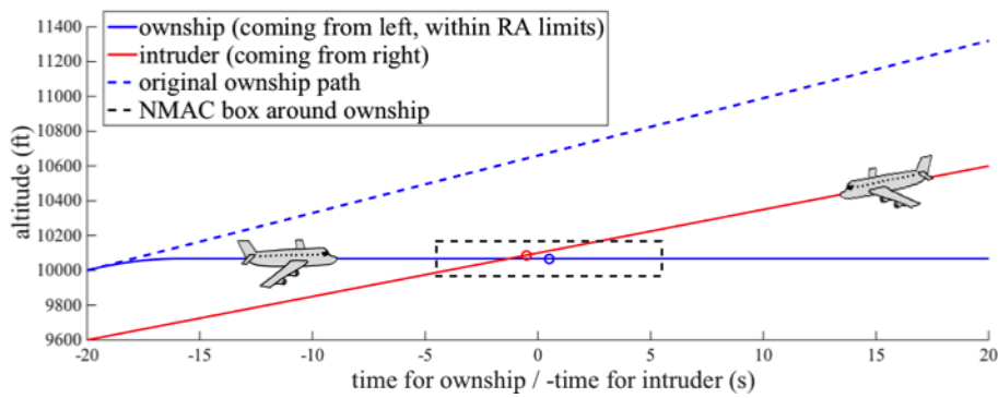
Fig. 14 Safe Counterexample. Original ownship path (cyan) and intruder path (red) vs. ownship responding to a do-not-climb (DNC) advisory issued by the ACAS X tables in starting state: r = 4,000 ft, r_v = 200 ft/s, \theta_v = 180^\circ , h = 600 ft, v = 1,980 ft/min, v_I = -1,500 ft/min. Time is shown counting from -20 s to time 0; the time of closest horizontal approach. The 2D projection of the NMAC cylinder is shown centered around the ownship as a dashed rectangle; the intruder intersecting with the NMAC region is shown by a red circle.
