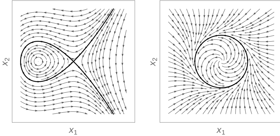
(a) Positive invariance of the variety V_{\mathbb{R}}(x_1^2 + x_2^3 - x_2^2) provable using FI (but not Lie since (0, 0) is a singular point).
