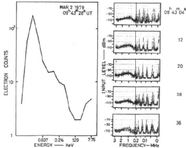
Fig.7. The energetic particle spectrum measured by ESP [19].
