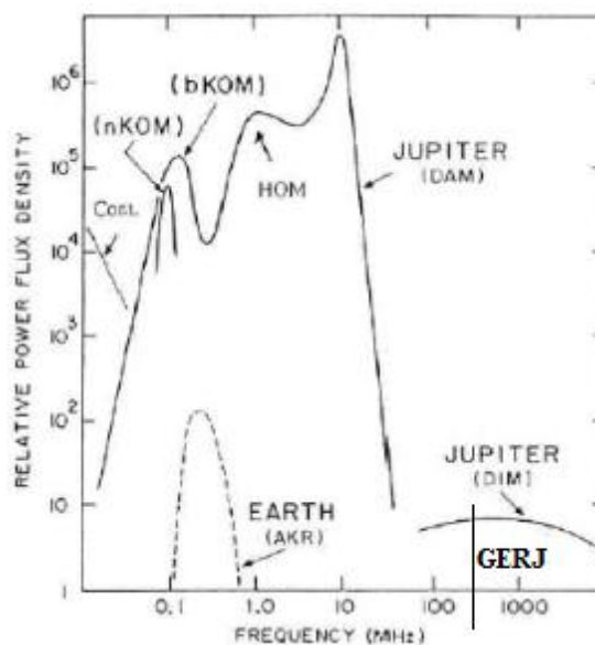
Fig. 5. Spectra of Jovian magnetospheric radiations. The power flux is normalized to constant distance. The spectrum of the Earth's is also shown as a comparison with Jupiter [17].
