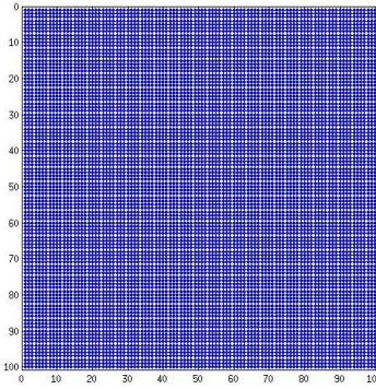
Figure 1: Matrix A of the academic illustration
