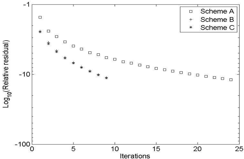
Figure 4: Residual convergence with the three refinement schemes in the Astrophysics application
