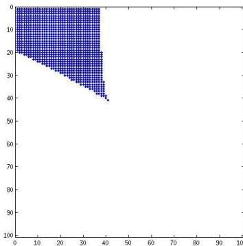
Figure 3: Matrix A of the Astrophysics application
