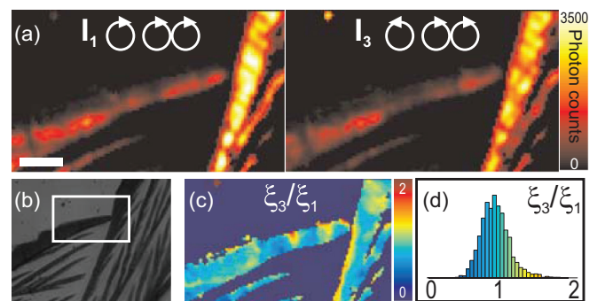
FIG. 1. (Color online) (a) SHG raw images of TTB crystals with dipolar ( \hat{e}_1\hat{e}_1\hat{e}_1 ) and octupolar ( \hat{e}_{-1}\hat{e}_1\hat{e}_1 ) polarization sets. (b) White light image and selected area for polarization-resolved SHG images. (c) Ratio between third and first orders (see text) and (d) its histogram. Scale bars: 10 \mu\text{m} .
