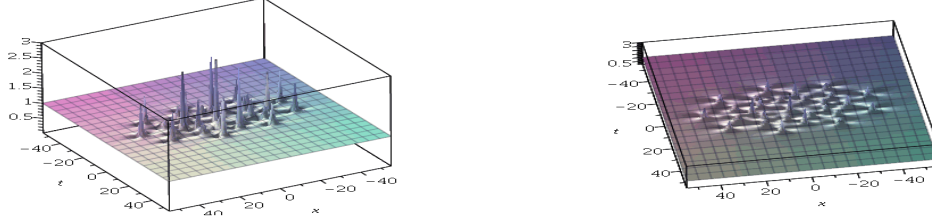
Figure 18: Solution to NLS, N=7 , \tilde{a}_4 = 10^{10} : 3 rings with 9 peaks, P_1 in the center; on the right, sight from top.
