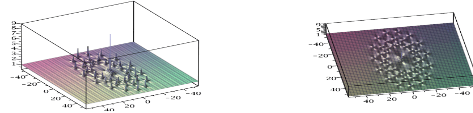
Figure 21: Solution to NLS, N=10 , \tilde{a}_7 = 10^{16} : 3 rings with 15 peaks, P_4 in the center; on the right, sight from top.
