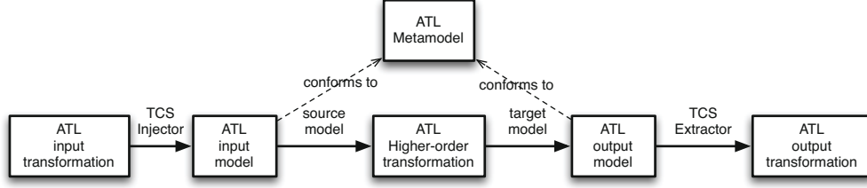
Fig. 3. An overview of Higher-Order transformation
