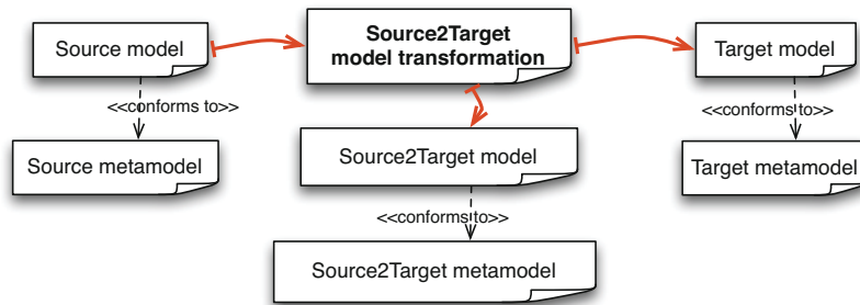
Fig. 2. The traceability mechanism
