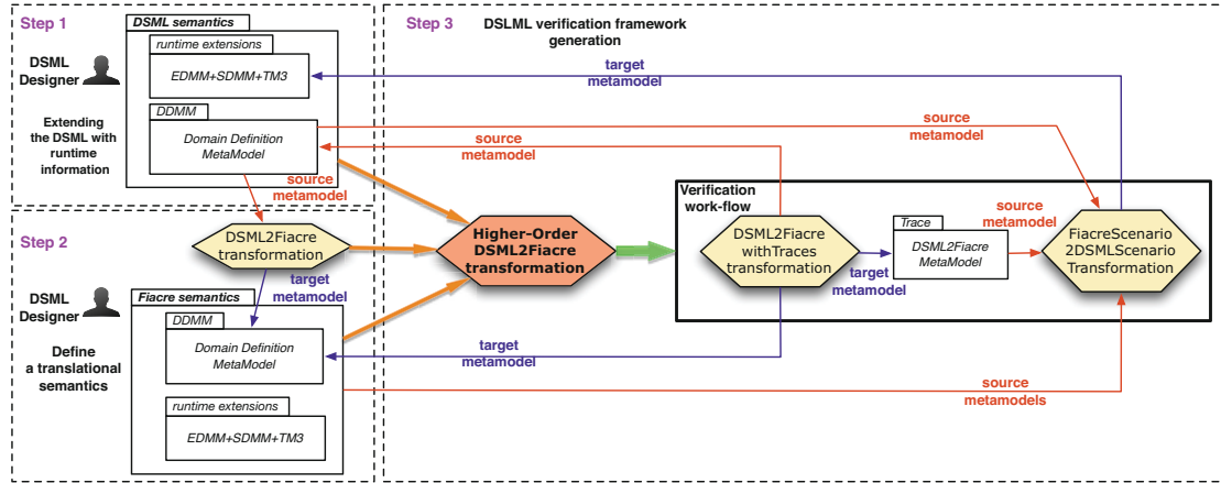
Fig. 4. Scheme of different steps to generate the DSML verification framework
