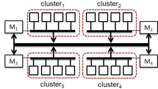
Fig. 4: A clustered architecture deploying a two-level hierarchical bus
