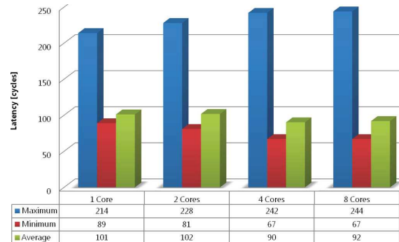
Fig. 2: Write memory access latencies in Freescale P4080
