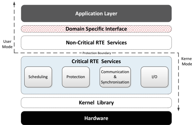
Fig. 3: parMERASA System Architecture
