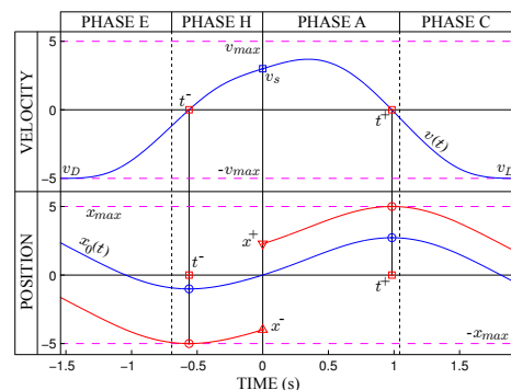
Fig. 5. Velocity and position (blue curves) around t = 0 . Saturated velocity variation is applied in order to determine the limits on initial positions (red triangles). Red curves are positions for these limits.
