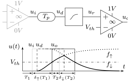
Figure 4: Simple analog channel model.
