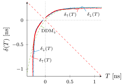
Figure 2: Measured \delta_{\downarrow} (blue) and \delta_{\uparrow} (red) for UMC-90 inverter chain for V_{DD} = 0.6 V , which support the involution hypothesis. By contrast, there is no perfect fit for the exponential DDM delay function (dashed green).
