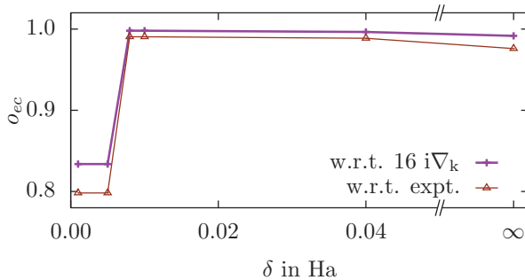
FIG. 4. (Color online) Overlaps of the normalized, mixed scGW RPA spectrum of CuGaSe 2 with the normalized i\nabla_{\mathbf{k}} spectrum for 16 \times 16 \times 16 k points and with the experimental one, as a function of \delta for a k -point mesh of 8 \times 8 \times 8 k points and for light polarization \parallel to the c axis.
