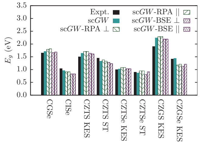
FIG. 14. (Color online) Optical band gaps from experiment, compared with the noninterpolated photoemission gaps calculated using the scGW method, and the optical gaps calculated using scGW -RPA and scGW -BSE, for \text{CuGaSe}_2 (CGSe), \text{CuInSe}_2 (CISE), \text{Cu}_2\text{ZnSnS}_4(\text{S,Se}) [CZTS, CZTSe], and \text{Cu}_2\text{ZnGeS}_4(\text{S,Se}) [CZGS, CZGSe] (see also Table II). KES and ST stand for kesterite and stannite structures, respectively.
