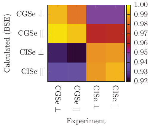
FIG. 13. (Color online) Overlap between experimental and scGW BSE spectra of \text{CuGaSe}_2 (“CGSe”) and \text{CuInSe}_2 (“CISE”).
