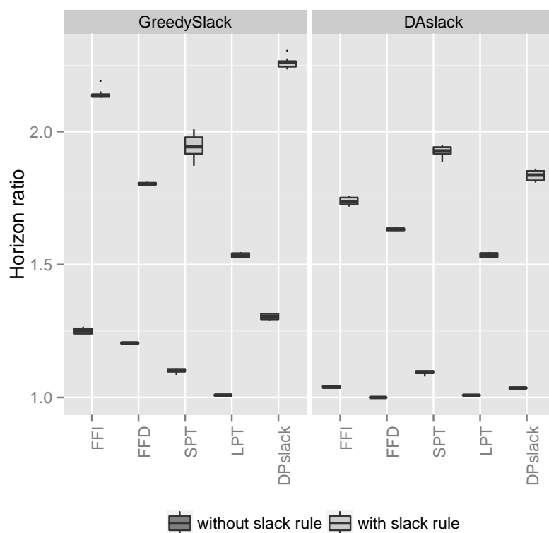
Figure 5: Horizon ratios of schedules generated with 10 sets of 10,000 jobs and 10 sets of 500 machines (100 instances). Each combination between a global and a local policy has an additional version that ignores the slack rule (left).
