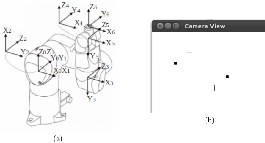
Fig. 9: Robot configuration for testing joint limits avoidance. a) Joint positions in deg: q_1 = 0 , q_2 = 90 , q_3 = -90 , q_4 = 0 , q_5 = 0 , q_6 = 0 . b) Simulated view, dots are the current feature locations and crosses are the desired locations.
