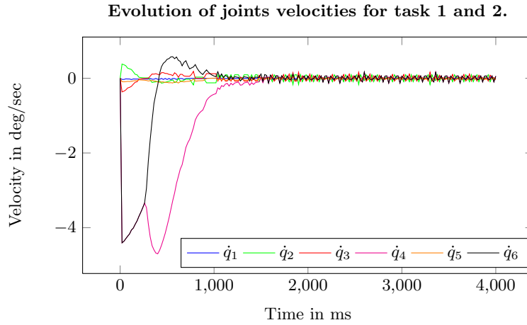
Fig. 11: Simulation of VS avoiding joint limits.
