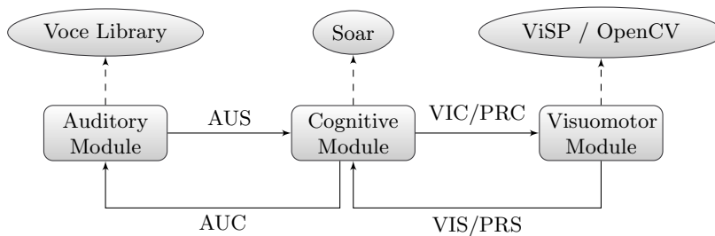
Fig. 2: The CRR architecture. The boxes represent modules and the ovals indicate the libraries wrapped inside the modules. The links between modules indicate topics. AUS: auditory sensory, PRS: proprioceptive sensory, VIS: visual sensory, AUC: Auditory command, VIC: Visual command, PRC: Proprioceptive command.
