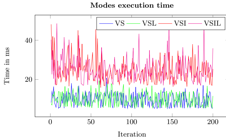
Fig. 8: Visuomotor module computing time.
