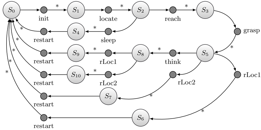
Fig. 4: The MDP task model. * = (\alpha, \rho) , where \alpha is the transition probability from s to s' when taking the action , and \rho is the reward associated with the state . From all actions there is a link to S_0 (omitted for clarity) modeling errors on the process with probability 1 - \alpha . The states are: S_0 : Started, S_1 : Initialized, S_2 : Object located, S_3 : Object reached, S_4 : Sleeping, S_5 : Object grasped, S_6 : Object released in location 1, S_7 : Object released in location 2, S_8 : Thinking, S_9 : Object released in location 1 after thinking, S_{10} : Object released in location 2 after thinking. The action a_0 initializes the system, a_1 signals the localization of the object, a_2 signals the robot to reach the object, a_3 puts the robot in sleeping mode, a_4 signals the robot to close the gripper, a_5 explores past events, a_6 and a_7 signal the robot to release the object at location 1 or 2 respectively, and a_8 restarts the system. If a state receives a negative feedback from the user \rho_i = -4 (punishment). In case of positive feedback, \rho_i = 2 (reward).
