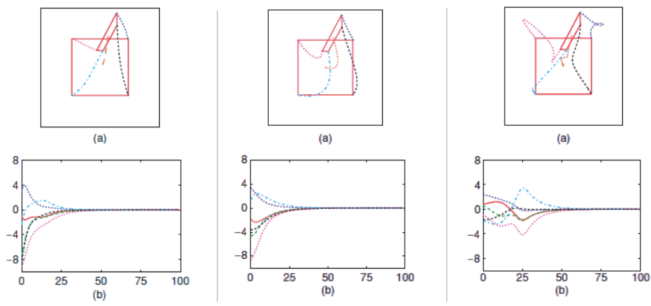
Fig. 1: Comparison between three IBVS (Image-base visual servoing) control schemes [8]. a) Initial and final position of the target on the camera image, and the trajectory followed by each point and the center of the virtual polygon. b) Evolution of V_C . From left to right the plots correspond to different calculations of the interaction matrix: L_e^+ (at each iteration), L_e^+ = L_{e^*}^+ (at equilibrium), and L_e^+ = (L_e^+ + L_{e^*}^+)/2 .
