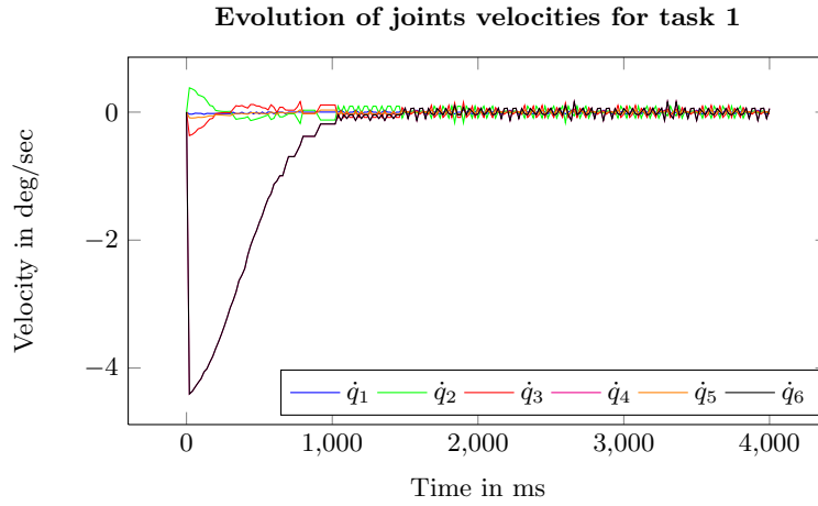
Fig. 10: Simulation of VS primary task.
