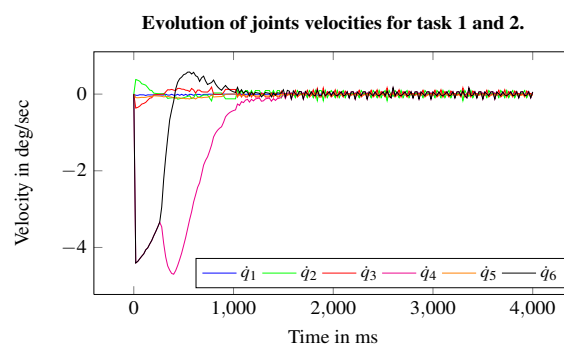
Figure 11: Simulation of VS avoiding joint limits.
