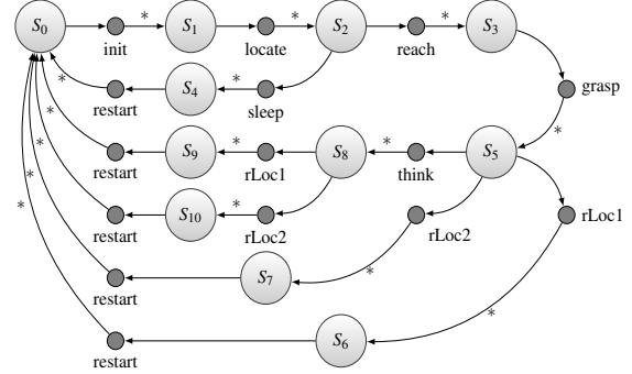
Figure 4: The MDP task model. * = (\alpha, \rho) , where \alpha is the transition probability from s to s' when taking the action , and \rho is the reward associated with the state . From all actions there is a link to S_0 (omitted for clarity) modeling errors on the process with probability 1 - \alpha . The states are: S_0 : Started, S_1 : Initialized, S_2 : Object located, S_3 : Object reached, S_4 : Sleeping, S_5 : Object grasped, S_6 : Object released in location 1, S_7 : Object released in location 2, S_8 : Thinking, S_9 : Object released in location 1 after thinking, S_{10} : Object released in location 2 after thinking. The action a_0 initializes the system, a_1 signals the localization of the object, a_2 signals the robot to reach the object, a_3 puts the robot in sleeping mode, a_4 signals the robot to close the gripper, a_5 explores past events, a_6 and a_7 signal the robot to release the object at location 1 or 2 respectively, and a_8 restarts the system. If a state receives a negative feedback from the user \rho_i = -4 (punishment). In case of positive feedback, \rho_i = 2 (reward).
