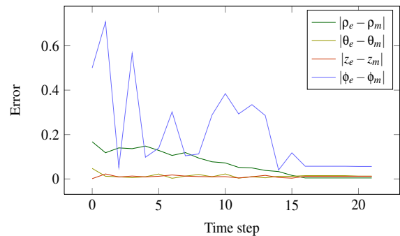
Figure 12: Evolution of the localization error between the estimations e and the measurements m .
