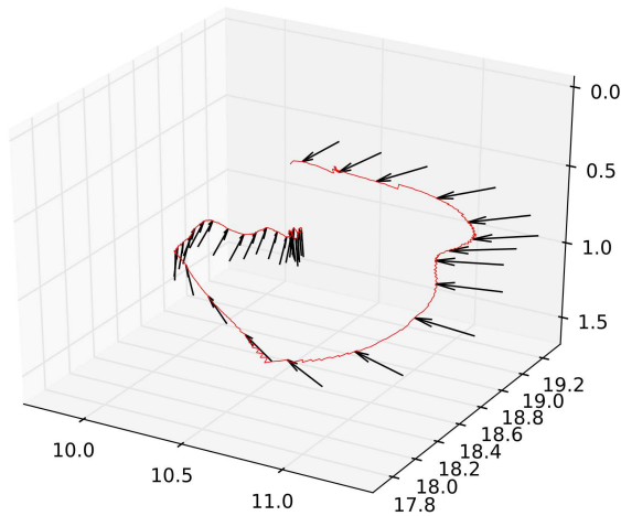
Fig. 13. Vehicle trajectory and orientation during a stabilisation trial. The initial yaw error is close to 180^\circ . This quasi-circular path is traced by the vehicle's center, while the camera stays oriented down on the target.
