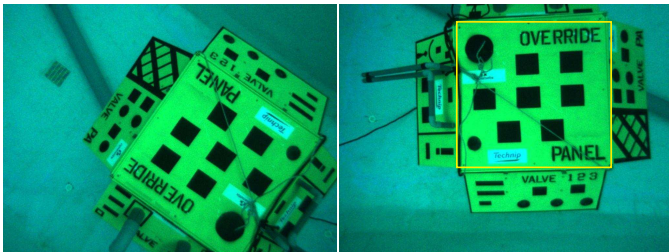
Fig. 10. Initial and final images of the simple stabilisation trial with the down-looking camera. Yellow rectangle marks the planar target of interests, where features are sought to be matched and compared with the reference. The initial heading error is of the order of 160^\circ .
