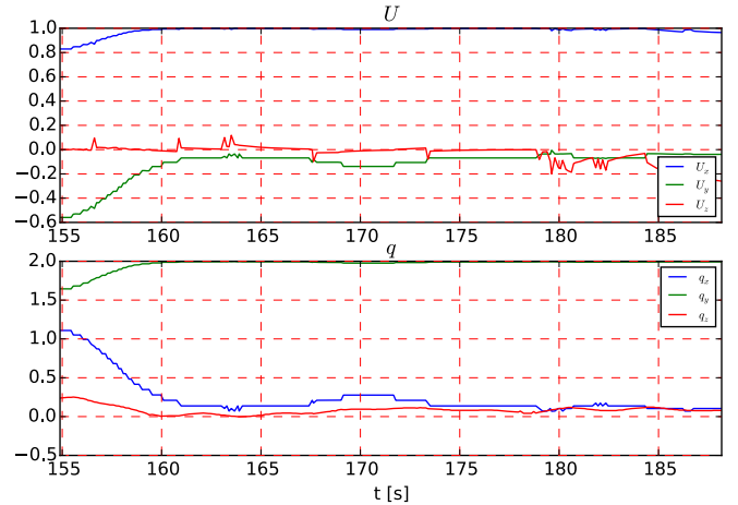
Fig. 6. Error variables U and q representing the pipe direction and transversal position in the AUV reference frame, respectively, during the pipe following exercise. They both quickly converge to and remain around their desired values: [1.0, 0.0, 0.0]^T and [0.0, 1.96, 0.0]^T respectively. The errors at t=185 s correspond to the false detections coinciding with the end of the test pipe.
