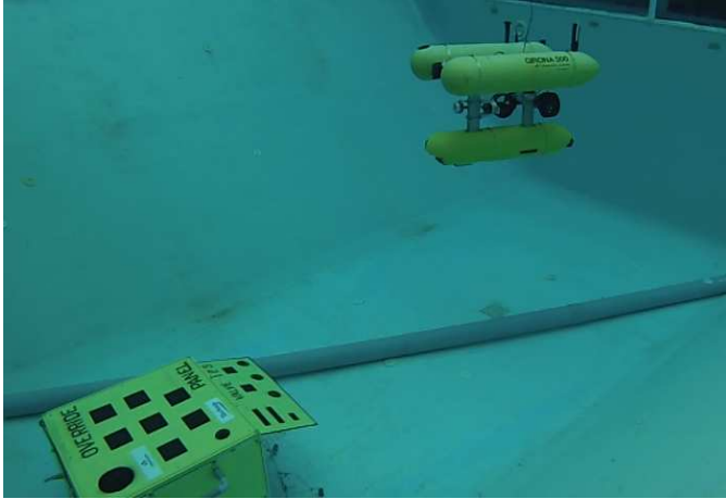
Fig. 5. AUV follows the mock pipeline. The mockup of a subsea manifold to be inspected is also visible in the photo.
