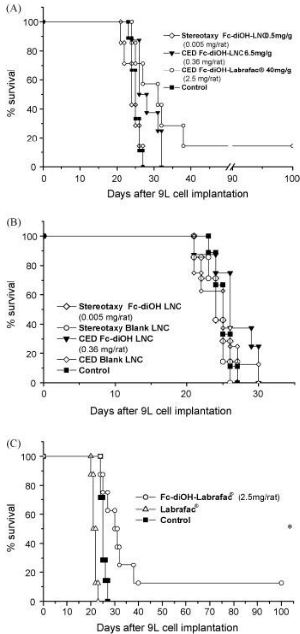
Fig. 4. Kaplan–Meier survival curves for 9L-glioma bearing rats for escalating doses of Fc-diOH encapsulated in LNCs or solubilised in Labrafac ® versus appropriate controls. (A) represents the survival curves in days after tumour implantation for untreated animals = control group (■-), stereotaxy of Fc-diOH-LNCs 0.005 mg/rat (◇-), CED of Fc-diOH-LNCs 0.36 mg/rat (▼-), and CED of Fc-diOH-Labrafac ® 2.5 mg/rat (○-). No significant differences were found between treatment with Fc-diOH-LNCs 0.005 mg/rat and 0.36 mg/rat versus blank LNCs administered in stereotaxy or by CED (B). The difference became significant only for the group treated with the highest dose (Fc-diOH-Labrafac ® 2.5 mg/rat) compared to the control group ( p = 0.018 ) and also to the group treated with Labrafac ® alone ( p < 0.0001 ) (C).
