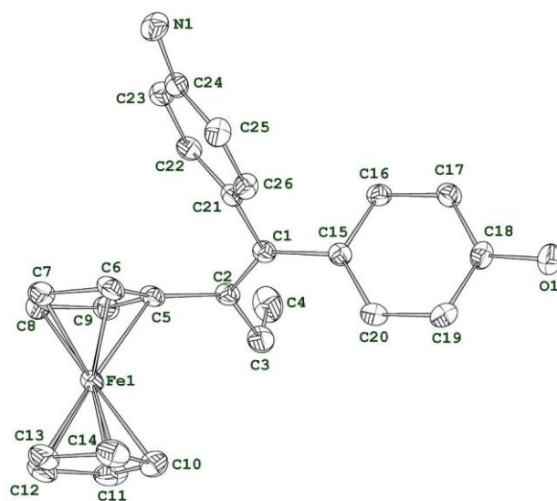
Figure 1. ORTEP diagram of ( E )- 7b . Thermal ellipsoids shown at 50% probability level, and hydrogen atoms have been omitted for clarity. Selected bond distances (Å) and bond angles (°): Fe1–C 9 =2.061(2), C1–C2=1.372(2), C18–O1=1.376(2), C24–N1=1.420(2), Fe1–
