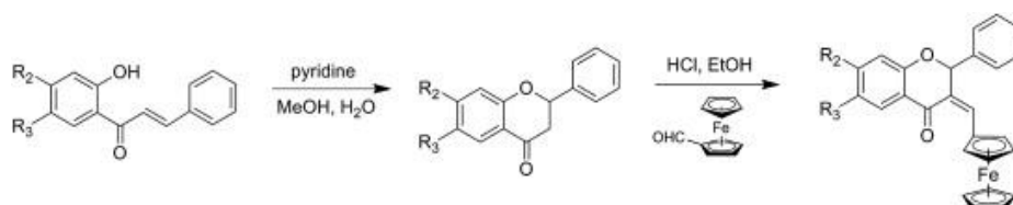
Scheme 2. Synthesis of ferrocenyl flavanones. 6a = unsubstituted; 6b : R_2 = OMe ; 6c : R_3 = OMe ; 6d : R_3 = Cl .
