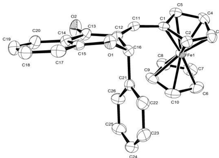
Fig. 1. Ortep diagram of 6a . Thermal ellipsoids shown at 50% probability, hydrogen atoms omitted for clarity. Selected bond distances (Å): C13–O2 = 1.224(2); Fe1–C Cp = 2.027(2)–2.049(2) (range), 2.036(2) (avg); C1–C11 = 1.439(3); C11–C12 = 1.339(3); and angles (°): Cp centroid –Fe–Cp centroid = 178.10°; C1–C11–C12 = 131.05(18)°; C13–C12–C16–O1 = -41.13^\circ .
