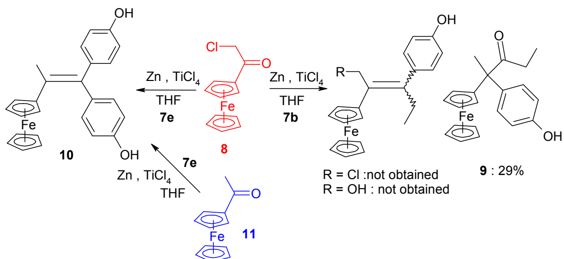
Scheme 3. McMurry reaction between 8 (or 11 ) and 7b or 7e .
