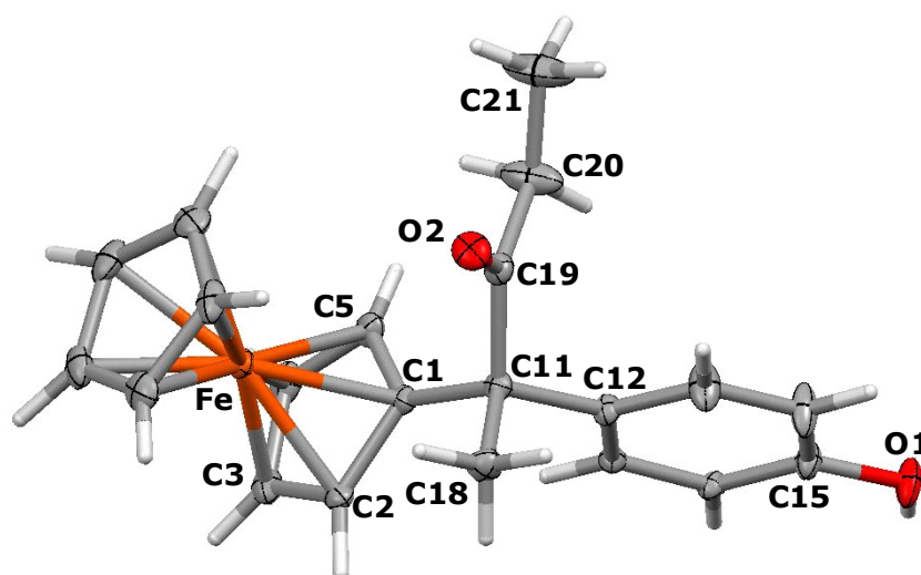
Figure 2. Molecular structure of 9 ; thermal ellipsoids are shown at 50% probability. Selected distances (Å): C(11)-C(1) 1.544(3), C(11)-C(18) 1.564(3), C(11)-C(12) 1.546(3), C(11)-C(19) 1.550(3), C(19)-C(20) 1.505(4), C(19)-O(2) 1.223(3), C(15)-O(1) 1.376(3), Fe-centroid(C 5 H 4 ) 1.664, Fe-centroid(C 5 H 5 ) 1.667.
